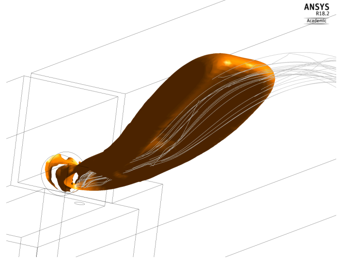
FIGURE 4: DPM PARTICLE TRACKS WITH LOCATION OF THE 0.9 CONTOUR OF PROGRESS VARIABLE
