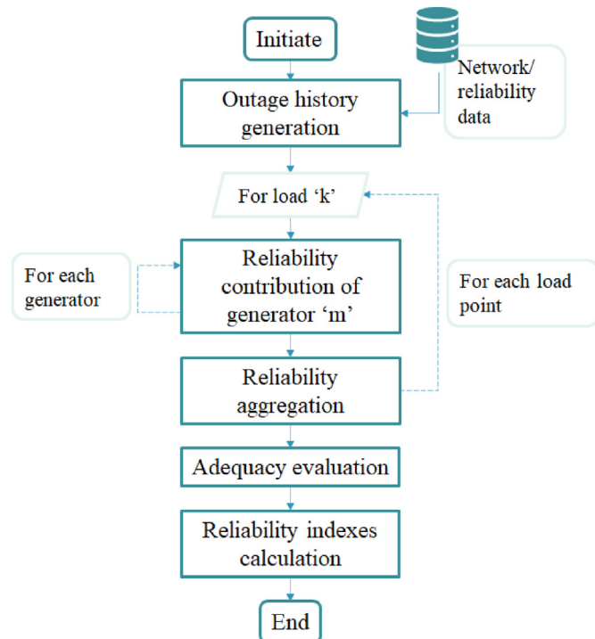
Fig. 2. General reliability evaluation considering multiple feeding paths and generation adequacy.
