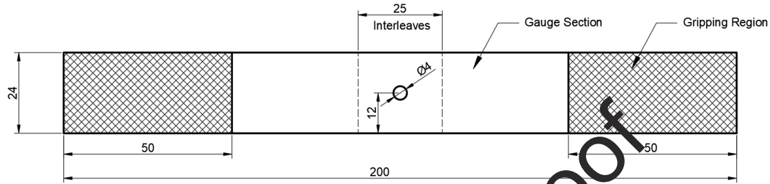
Fig.1 Open-hole specimen configuration (Unit: mm)
