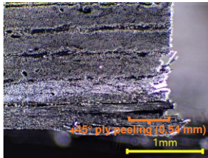
Interleaved sample with damage at drill site
