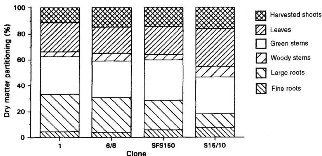
Figure 3. The proportion of dry matter partitioned to harvested shoots, leaves, green stems, woody stems, large roots and fine roots for each of four fully irrigated clones between December 1989 and November 1990. The absolute values for dry matter are given in Table 6.
