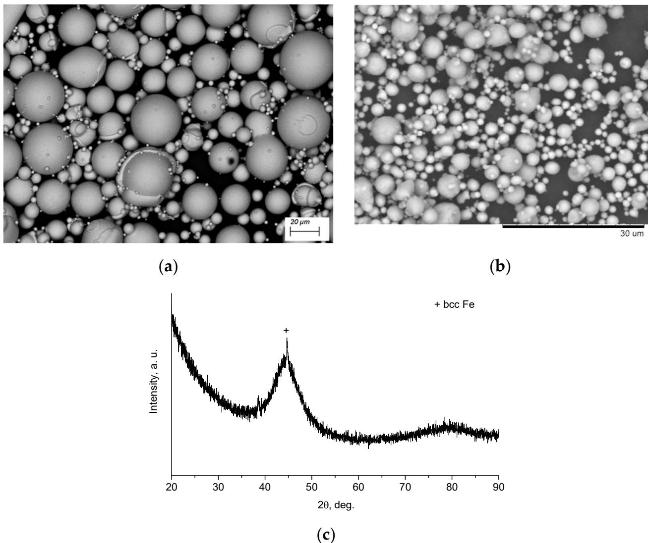
Figure 1. (a) Scanning electron microscopy (SEM) image of the \text{Fe}_{66}\text{Cr}_{10}\text{Nb}_5\text{B}_{19} metallic glass powder, back-scattered electron (BSE) image, (b) SEM image of the aluminum powder, back-scattered electron image, (c) X-ray diffraction (XRD) pattern of the \text{Fe}_{66}\text{Cr}_{10}\text{Nb}_5\text{B}_{19} metallic glass powder. The minor phase in the alloy is body-centered cubic iron (bcc-Fe).
