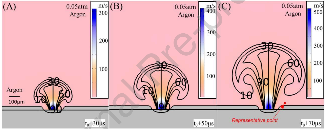
Fig.6 Color contour denotes velocity distribution of vapor plume flow and vapor-induced gas flow during PBF-LB of 316L powders. The isoline indicates the mass fraction of the plume. Four concentration levels are labeled along the decreasing direction from the plume core to the plume boundary, i.e., 90%, 60%, 30%, and 10%, respectively. t_0=372\text{ }\mu\text{s} corresponding to the beginning of evaporation. Fig.6A, Fig.6B, and Fig.6C show the velocity field of vapor plume flow and vapor-induced gas flow, and the mass fraction of vapor plume in 0.05atm argon at t_0+30\text{ }\mu\text{s} , t_0+50\text{ }\mu\text{s} , and t_0+70\text{ }\mu\text{s} , respectively.
