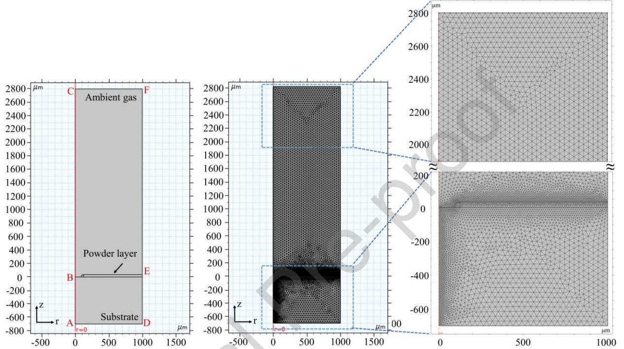
Fig.2 Geometry and mesh discretization of the proposed Thermal-Fluid-Evaporation model.
