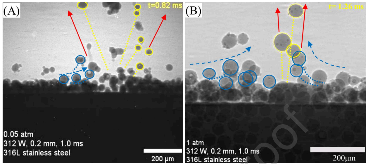
Fig.7 In-situ observation of power spattering and denudation during PBF-LB of 316L powders. (A) X-ray image showing spattering and denudation in 0.05 atm argon. (B) X-ray image showing spattering and denudation in 1 atm argon. X-ray images are taken from the supplementary videos of [7]. Parameters for PBF-LB experiments are same to these in Section 3.2.
