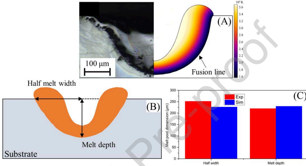
Fig.3. Validation of the proposed computational model. (A) Comparison of melt pool morphology between experimental observation [29] and simulated result. (B) Schematic sketch of the melt pool in keyhole mode and the dimension definition. (C) Quantitative validation of experimentally observed and calculated dimensions. Material: IN625; Parameters: laser power of 700 W, laser radius of 102.5 \mu m, and pulse duration time of 3 ms.
