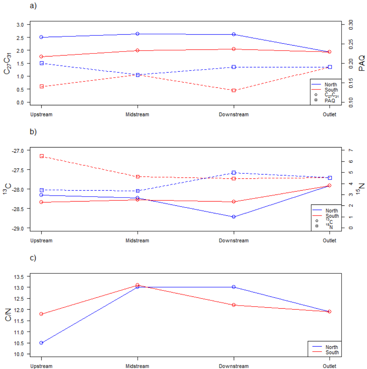
19 Fig. 5 Spatial variability of a) n -alkane proxies b) stable isotopes and c) C/N ratio in a 20 downstream direction in the two subcatchments. Each data point at upstream, midstream and 21 downstream location and the catchment outlet represents a composite of three individual river- 22 bed sediment samples.
