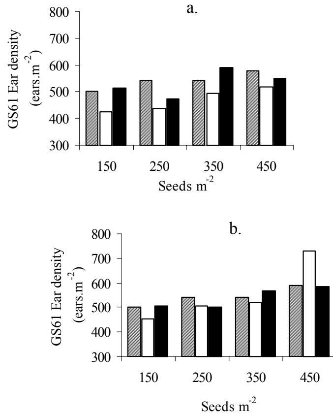
Fig. 20. Seed rate vs. ear density at GS61 for the standard and variable strips compared with desired target density for a. ON00 and b. FH00 : \square , Standard; \blacksquare , Variable; \hatched , Target
