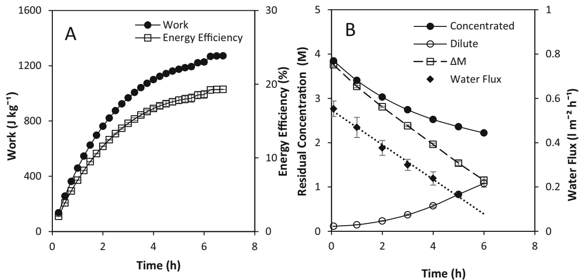
Fig. 4. (A) Energy efficiency and work recovered over time, and (B) water flux and feed concentration profile over time from 250 g of 4 M and 250 g of 0.02 M in recycle. Feed flow rate, 200 ml min -1 ; feed temperature 25 °C; current 100 mA.
