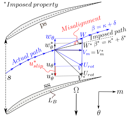
FIGURE 4: OVERVIEW OF CORRECTION FORCE MODEL VELOCITY COMPONENTS DUE TO FLOW MISALIGNMENT WITH RESPECT TO THE IMPOSED RELATIVE PATH.
