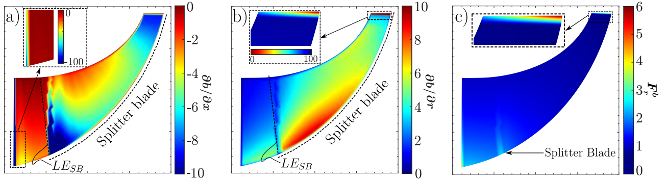
FIGURE 10: SRV2 IMPELLER A) AXIAL AND B) RADIAL BLOCKAGE GRADIENT TERM DISTRIBUTIONS, C) RADIAL COMPONENT OF SUBSIDIARY FORCE RELATED TO BLOCKAGE GRADIENT TERMS.
