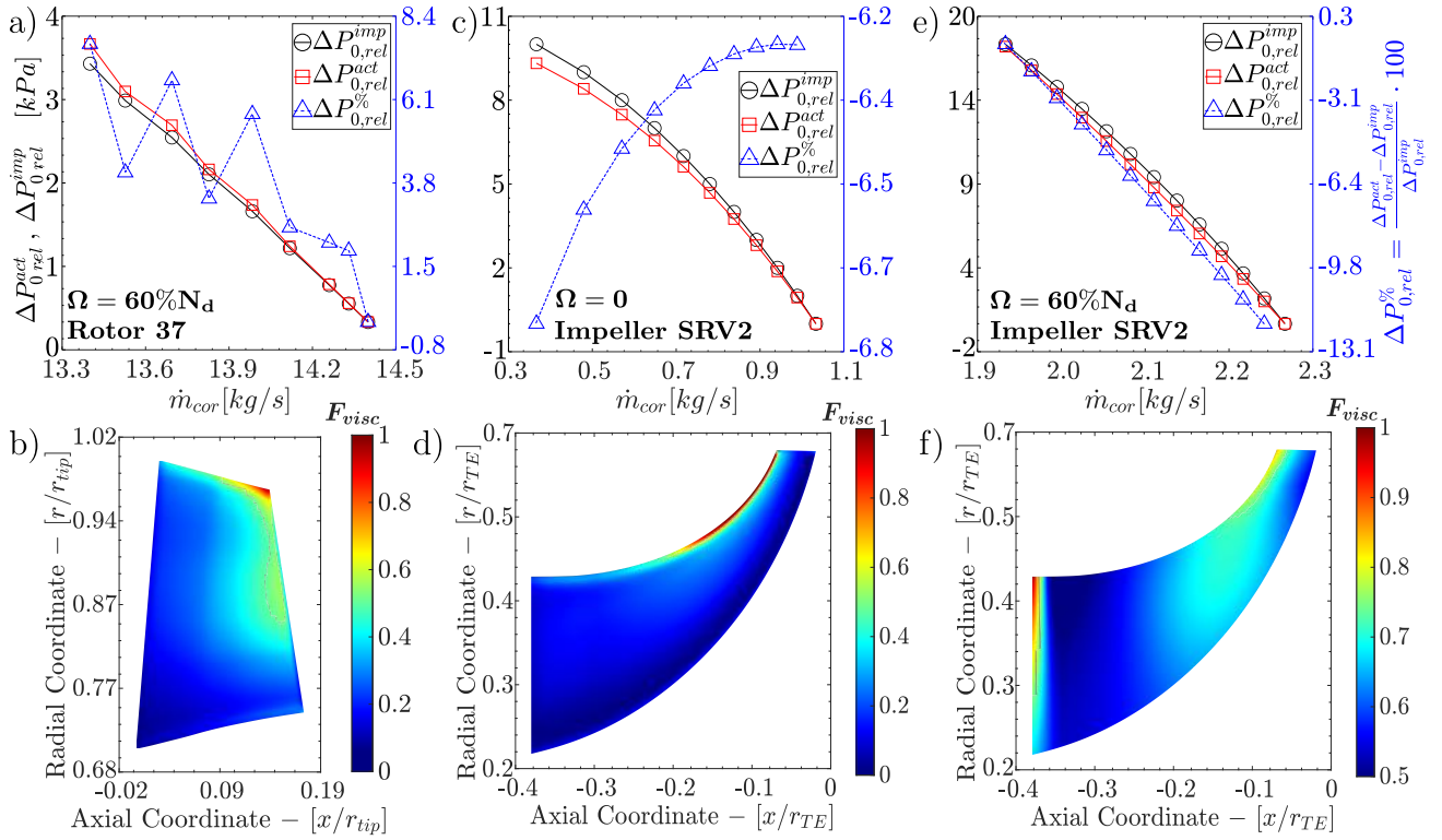
FIGURE 14: COMPARISON OF IMPOSED VS. ACTUAL TOTAL PRESSURE LOSS AND VISCOUS FORCE DISTRIBUTION IN BLADE PASSAGES OF ROTOR 37 (LEFT) AND IMPELLER SRV2 WITH UNIFORM (MIDDLE) AND CFD-EXTRACTED DISTRIBUTION COEFFICIENT (RIGHT).
