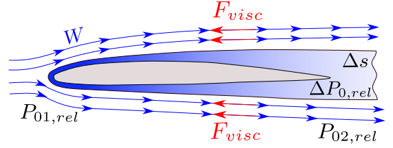
FIGURE 5: VISCOUS FORCE ACTING PARALLEL AND OPPOSITE ALONG A RELATIVE STREAMLINE GENERATING ENTROPY AND PRESSURE LOSS.
