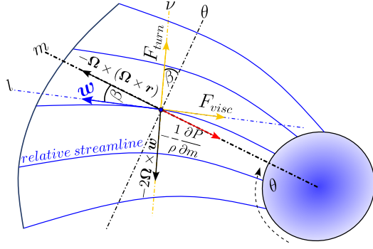
FIGURE 3: FORCE BALANCE ALONG A RELATIVE STREAMLINE INSIDE A ROTOR.
