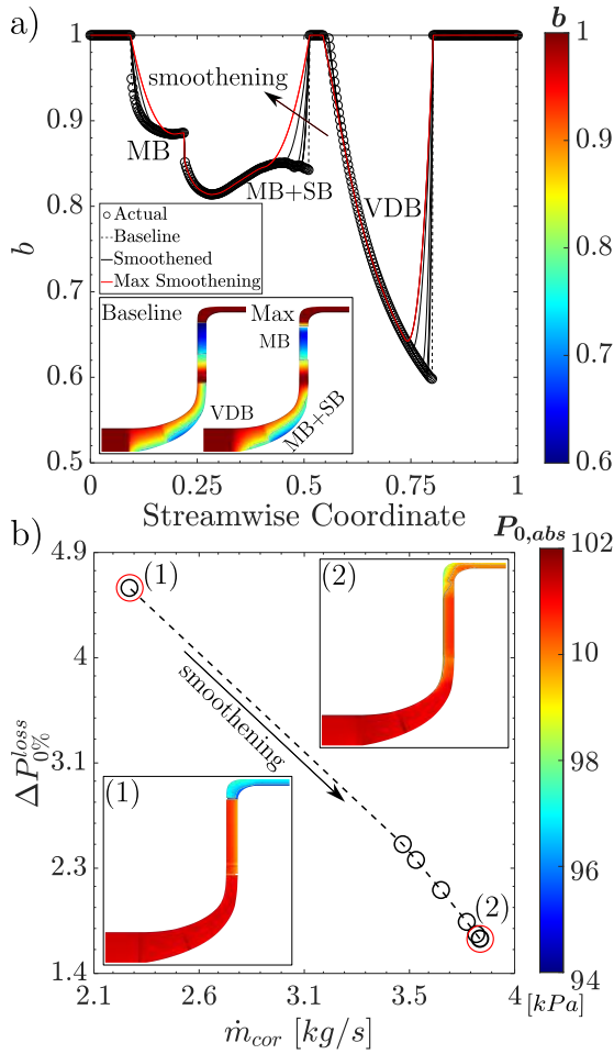
FIGURE 11: A) ACTUAL AND MODIFIED BLOCKAGE DISTRIBUTIONS OF NASA CC3 COMPRESSOR AND B) TOTAL PRESSURE LOSS FOR DIFFERENT LEVELS OF BLOCKAGE SMOOTHENING.
