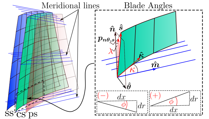
FIGURE 2: BLADE SURFACE GRIDS AND DEFINITION OF BLADE ANGLES AND VECTORS FOR THE EVALUATION OF THE BLADE CURVATURE.
