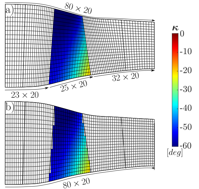
FIGURE 1: BLADE ANGLE DISTRIBUTION AND COMPUTATIONAL DOMAIN OF ROTOR 37 [27] FOLLOWING A) GEOMETRY-ADAPTIVE AND B) UNIFORM APPROACH.
