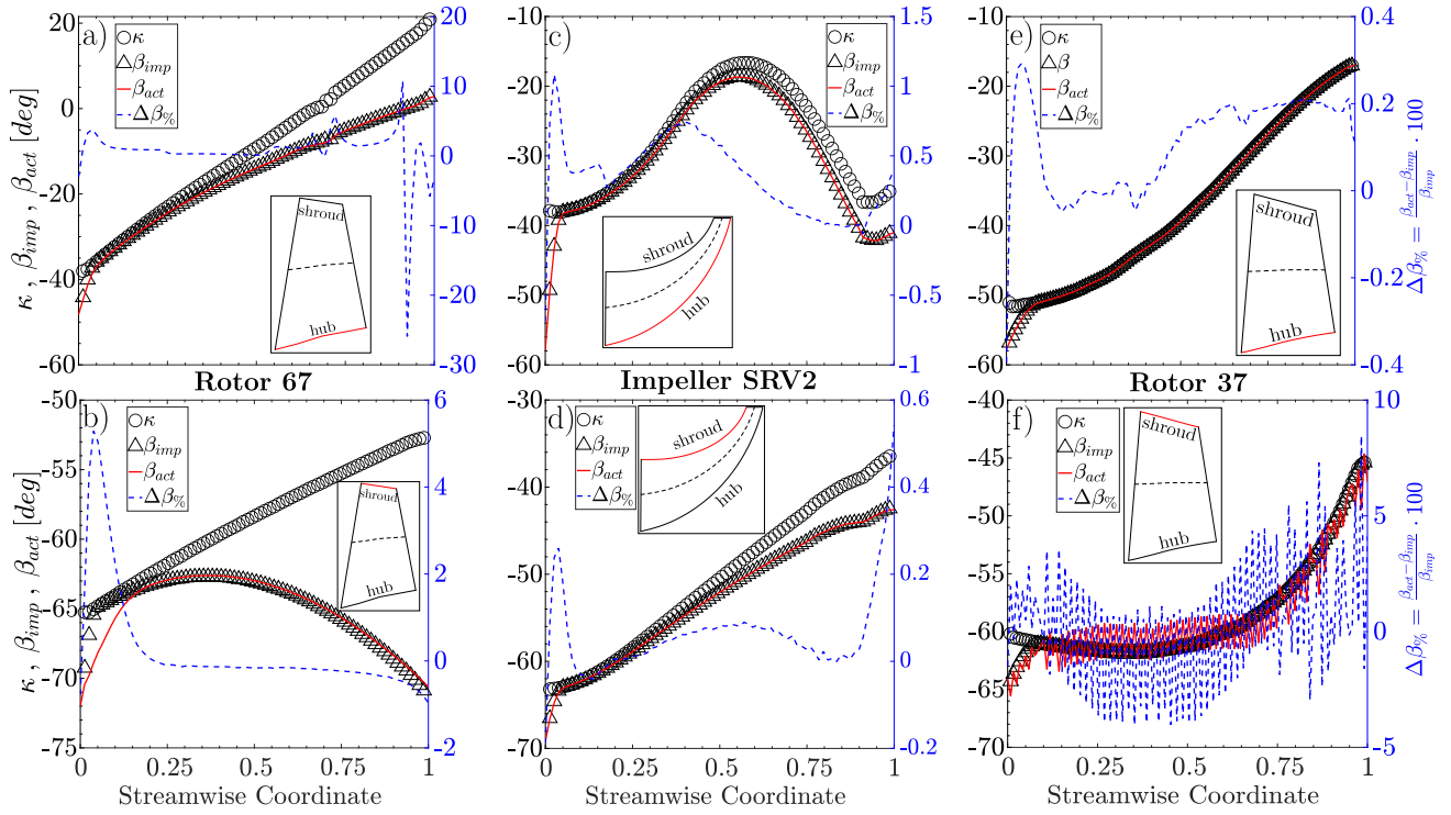
FIGURE 13: MERIDIONAL DISTRIBUTION OF BLADE ANGLE (CIRCLES), IMPOSED FLOW ANGLE (TRIANGLES) AND ACTUAL FLOW ANGLE AT HUB AND SHROUD OF ROTOR 67, IMPELLER SRV2 AND ROTOR 37.
