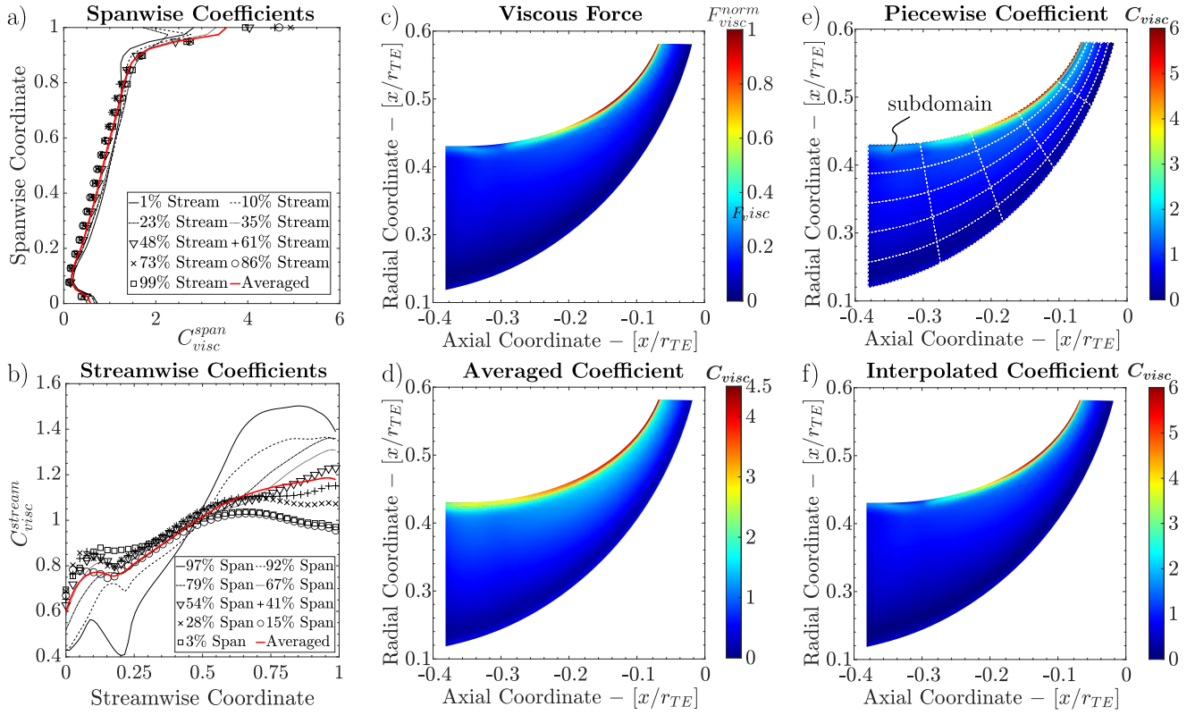
FIGURE 7: A) SPANWISE AND B) STREAMWISE DISTRIBUTION COEFFICIENTS AT DIFFERENT STREAMWISE AND SPANWISE LOCATIONS RESPECTIVELY, C) CFD-EXTRACTED VISCOUS FORCE DISTRIBUTION AND VISCOUS FORCE COEFFICIENTS DERIVED FOLLOWING THE D) AVERAGE, E) PIECEWISE AND F) INTERPOLATED CELL-BASED APPROACH.
