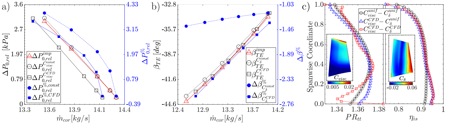
FIGURE 15: COMPARISON OF IMPOSED AND ACTUAL A) LOSSES AND B) FLOW ANGLES DOWNSTREAM OF R37 TE USING UNIFORM AND CFD-DERIVED DISTRIBUTION COEFFICIENTS. SPANWISE PROFILE OF PR_{tt} AND \eta_{is} OBTAINED WITH DIFFERENT COEFFICIENTS (C).
