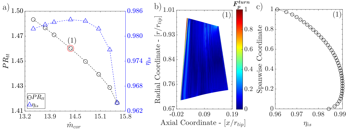
FIGURE 9: A) 'ISENTROPIC' PRESSURE AND EFFICIENCY CHARACTERISTICS OF ROTOR 37 AT 60% SPEED, B) DISTRIBUTION OF SUBSIDIARY PARALLEL FORCE AND C) SPANWISE ISENTROPIC EFFICIENCY DISTRIBUTION DOWNSTREAM THE TE.
