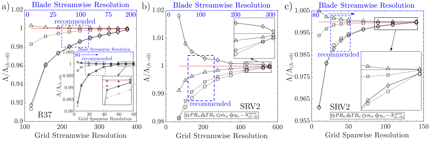
FIGURE 8: STREAMWISE AND SPANWISE GRID SENSITIVITY ANALYSIS: ROTOR 37 (A) AND IMPELLER SRV2 (B, C).
