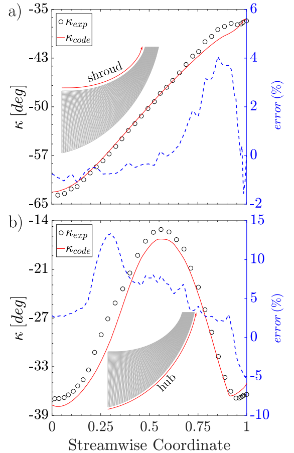
FIGURE 12: COMPARISON OF EXPERIMENTAL AND ESTIMATED BLADE ANGLE DISTRIBUTIONS AT (A) SHROUD AND (B) HUB OF IMPELLER SRV2.
