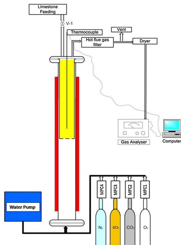
Fig. 1 – Bubbling bed test facility.
