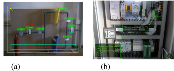
Figure 17. (a) View through HMD of a helium flushing system (mockup) from Klinker [41]. (b) View of an electrical cabinet through HMD or HMD adapted from Wojcicki [35].
