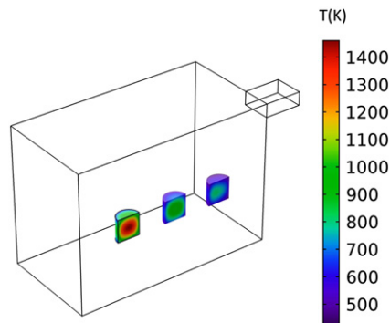
Fig. 10. Temperature distribution (K) in the three biomass samples placed after 600s at different locations along the centerline of the microwave cavity for input power of P = 800 W.
