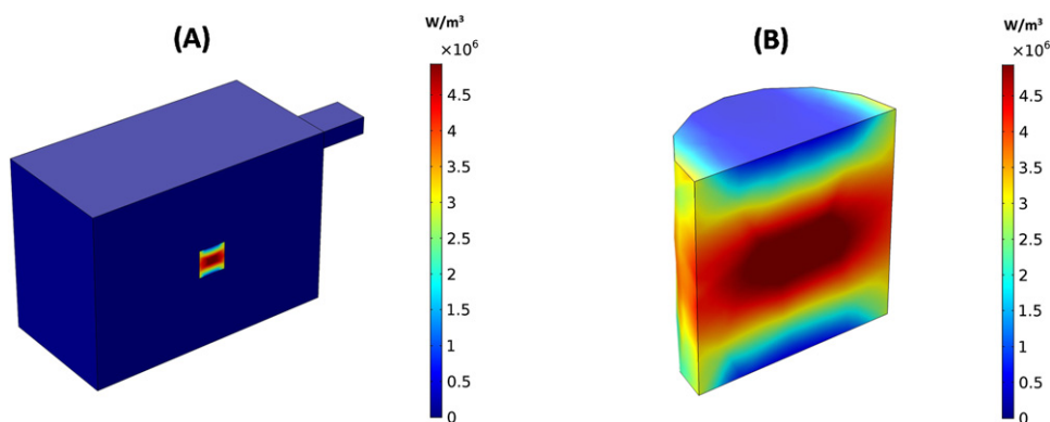
Fig. 3. Electromagnetic power loss density ( \text{W/m}^3 ) at applied input power P_o = 1200 \text{ W} in the entire microwave cavity with the biomass sample (A) and zoomed view of electromagnetic power loss density in the biomass sample alone (B).
