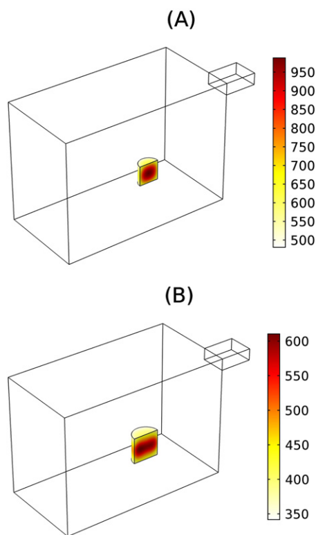
Fig. 9. Temperature distribution (K) in the biomass bed for two different sample sizes at applied input power of P_0 = 800 W after 600s.
