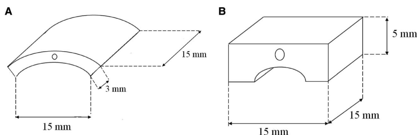
2 Test samples drawing: a curve shape, b bridge shape
