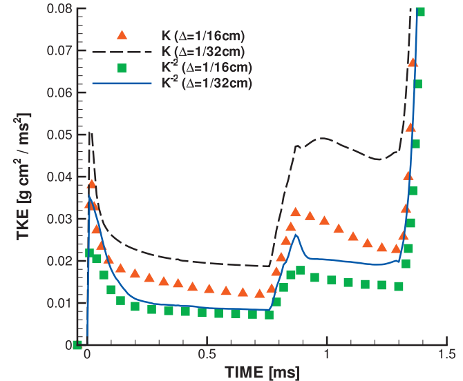
FIG. 9. (Color) Evolution of total turbulent kinetic energy for different perturbation spectra and grid resolutions.
