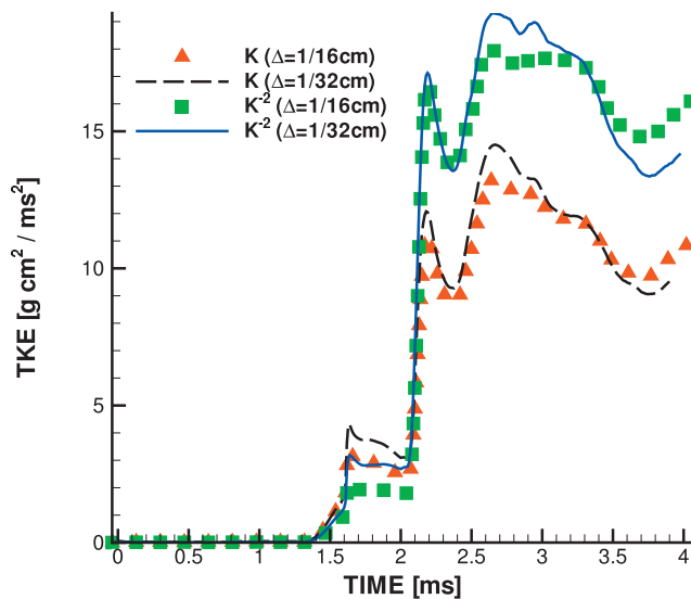
FIG. 9. (Color) Evolution of total turbulent kinetic energy for different perturbation spectra and grid resolutions.
