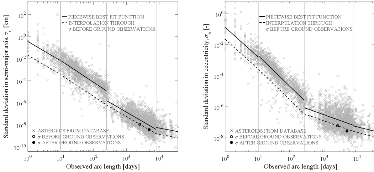
Fig. 5. Keplerian element uncertainty for asteroid 2005 WD before and after collecting ground-based observations
