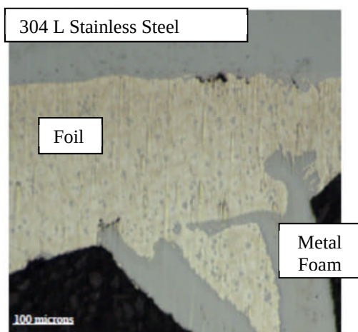
Figure 6 - Micrograph of laser braze joint of stainless steel to 1116 Grade foam
