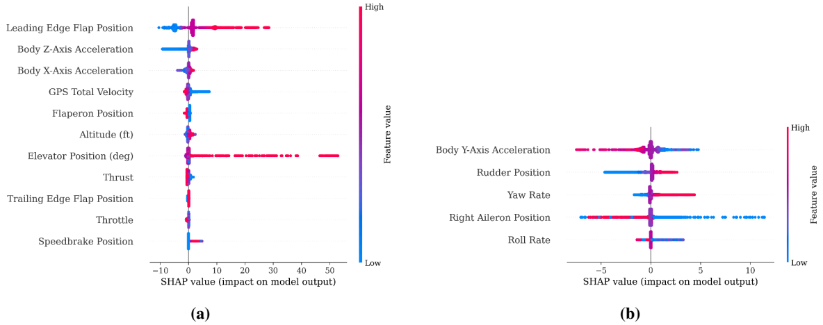
Fig. 8 SHAP values for (a) the angle of attack and (b) the sideslip angle
