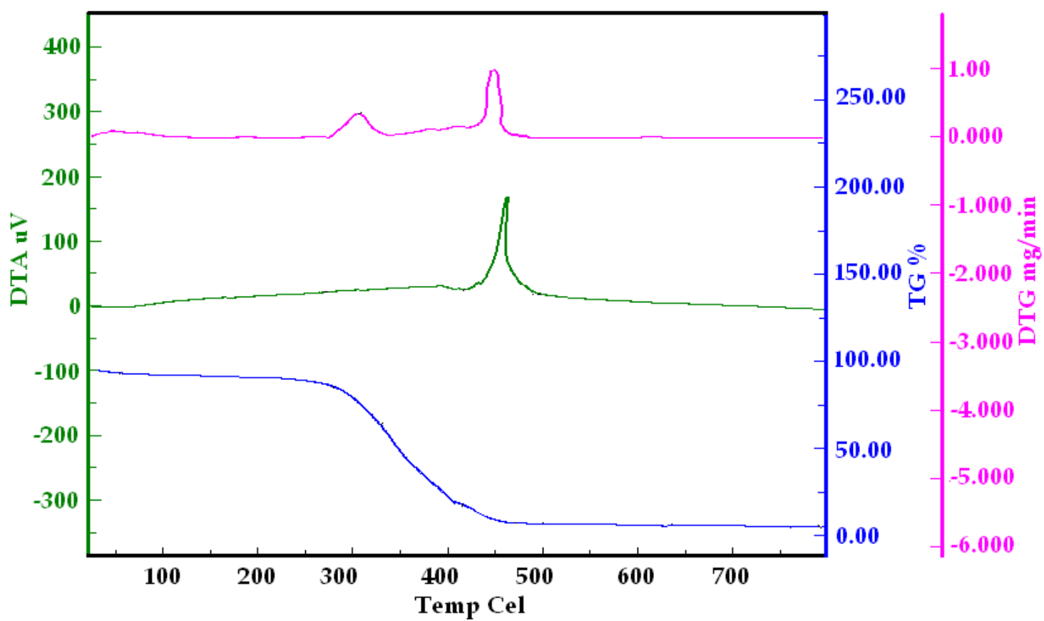
Figure 8 (b) - Thermogravimetric analysis of silane treated cellulosic Eulaliopsis binata fibers
