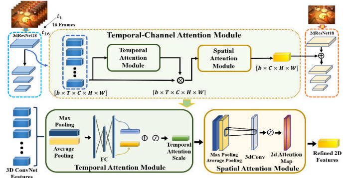
Fig. 3. Temporal-channel attention (TCA) module between the 3D ConvNet and 2D ConvNet. The TCA fusion contains two attention modules, namely a temporal attention module (TAM) and a spatial attention module (SAM).
