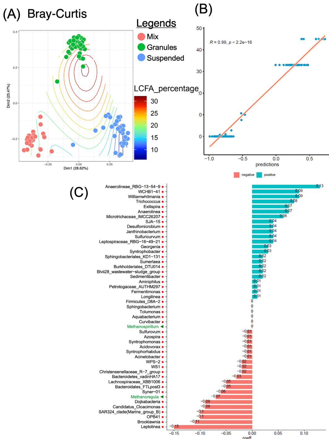
Fig. 4. a) Beta diversity contour plot with LCFA% regressed against the scores of the ordination (PCoA) using Generalised Additive Model (GAM); b) \beta – coefficients returned from CODA-LASSO procedure as two disjoint sets (those that are positively related, and those that are negatively related with the LCFA%) c) The predictions from the fitted model through CODA-LASSO was then further regressed against the true LCFA % to show agreement.
