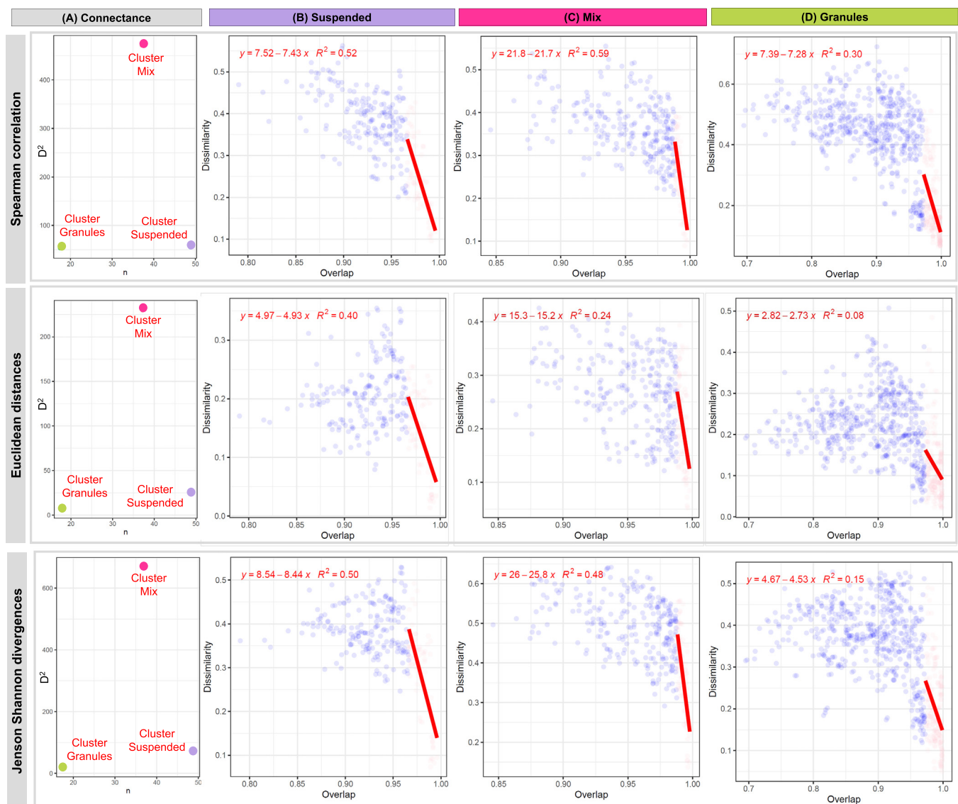
Fig. 6. Complexity-stability relationship of clusters (suspended, Mix, granular) where, (a) the effective connectance ( D^2 ) is calculated based on fitting a linear regression to top 25 % overlap values for (b) cluster suspended, (c) cluster mix, (d) cluster granular using Jenson-Shannon divergences, Euclidean distances and Spearman correlation values.
