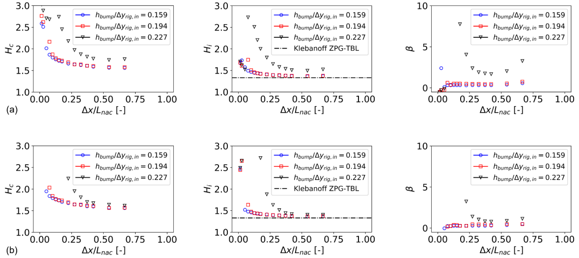
Fig. 18 Effect of change in bump height on boundary layer characteristics on the nacelle aeroline at mid-span ( \Delta z = 0 ). RANS computations with (a) k\omega - SST and (b) \gamma - Re_\theta turbulence models
