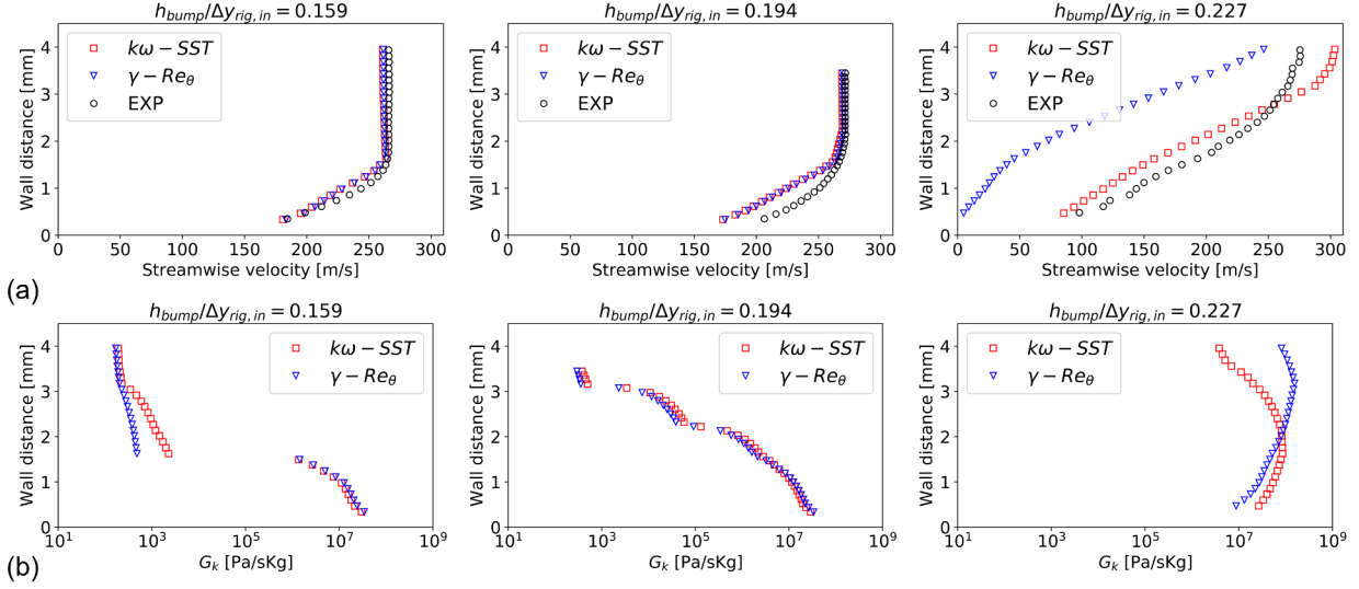
Fig. 17 Effect of change in bump height on (a) streamwise velocity and (b) modelled G_k distributions within the boundary layer on the nacelle aeroline at \Delta x/L_{nac} \approx 0.13 and \Delta z = 0
