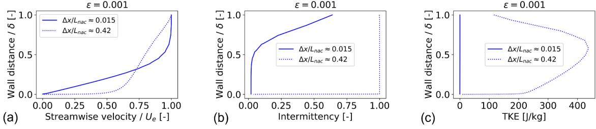
Fig. 19 (a) Non-dimensional streamwise velocity, (b) intermittency and (c) turbulent kinetic energy distributions across two boundary layers on the nacelle aeroline at mid-span ( \Delta z = 0 ) ahead ( \Delta x/L_{nac} \approx 0.015 ) and downstream ( \Delta x/L_{nac} \approx 0.42 ) of the shock. The y-axis in (a), (b), (c) and the x-axis in (a) were rescaled with the thickness ( \delta ) and the outer edge velocity ( U_e ) of each individual boundary layer. h_{bump}/\Delta y_{rig,in} = 0.227 . RANS computations with \gamma - Re_\theta turbulence model
