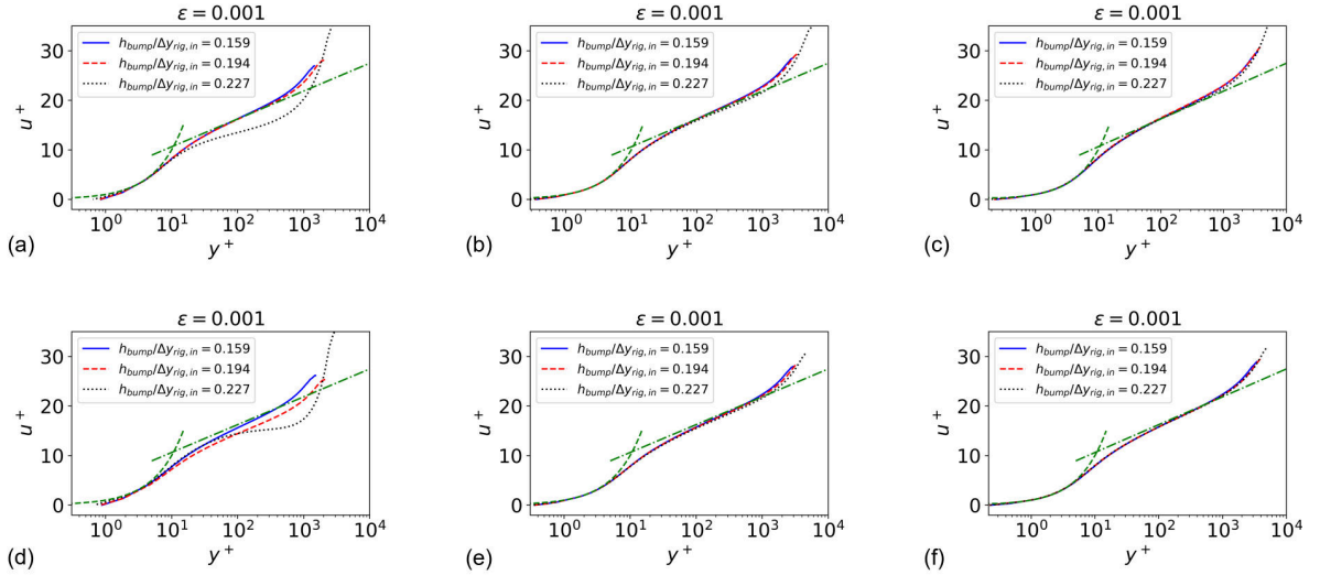
Fig. 20 Effect of change in bump height on the boundary layer on the nacelle aeroline at mid-span ( \Delta z = 0 ). (a), (d) \Delta x/L_{nac} \approx 0.22 ; (b), (e) \Delta x/L_{nac} \approx 0.54 ; (c), (f) \Delta x/L_{nac} \approx 0.67 . RANS computations with (a), (b), (c) k\omega - SST and (d), (e), (f) \gamma - Re_\theta turbulence models. Green dashed line: linear region ( u^+ = y^+ ); dotted-dashed green line: log region ( u^+ = \frac{1}{0.41} \ln(y^+) + 5.0 )
