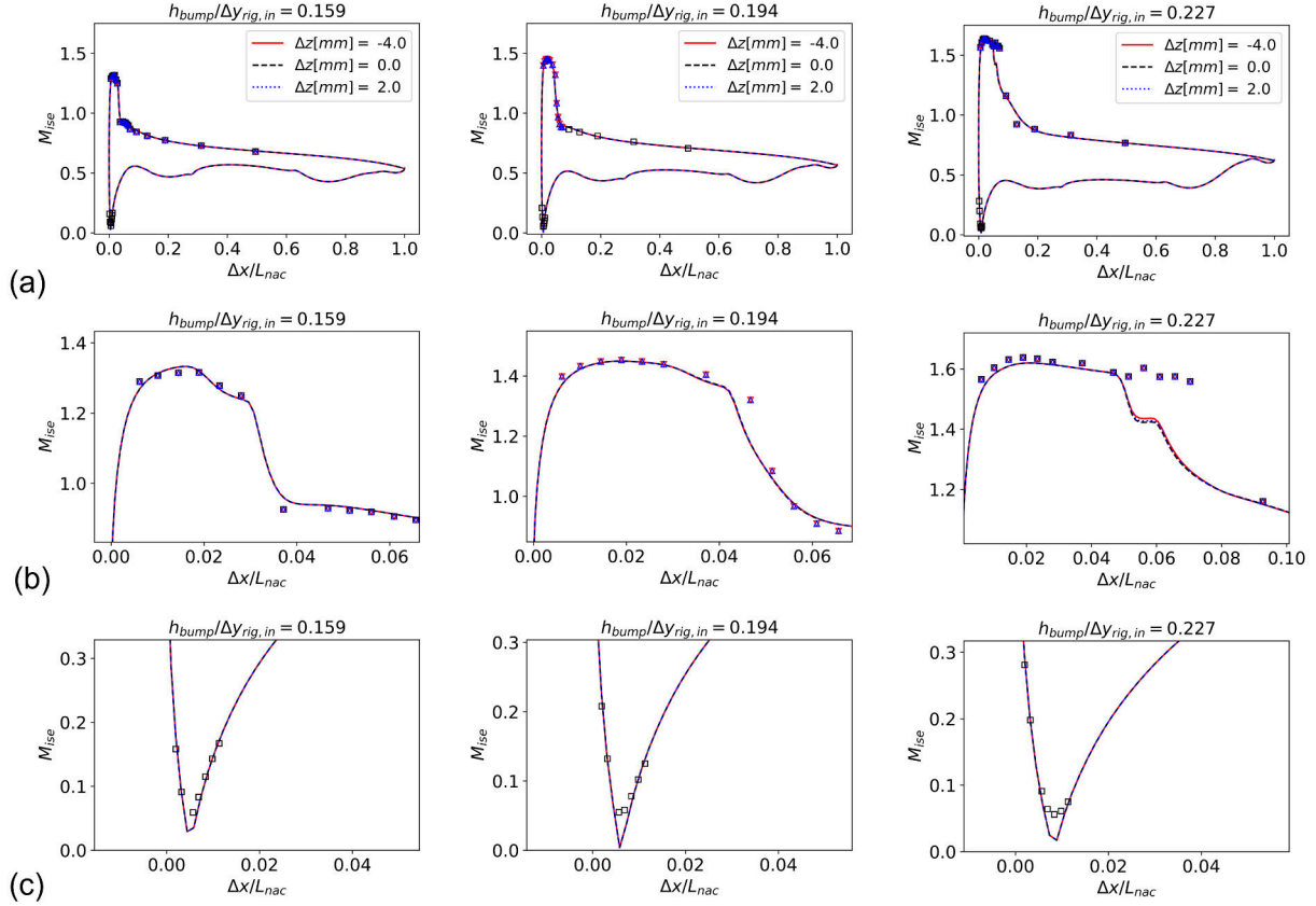
Fig. 14 (a) Effect of change in bump height on M_{ise} distribution on the nacelle aeroline at mid-span ( \Delta z = 0 ); (b) and (c) details of shock and stagnation point region, respectively. Lines: RANS computations with \gamma - Re_\theta ; Markers: experiments
