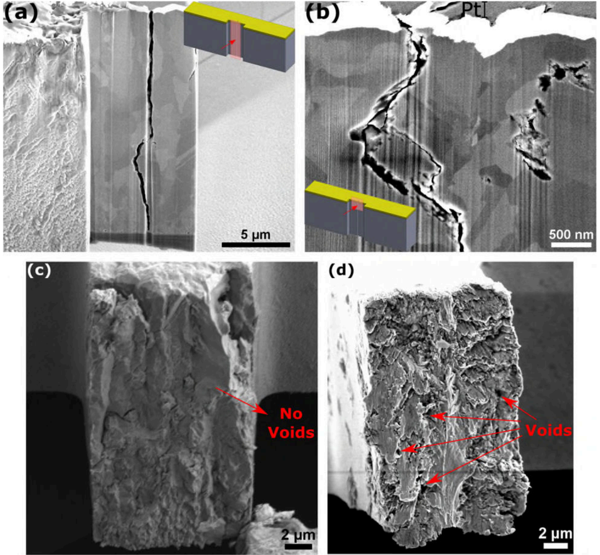
Figure 6. (a) Vertical FIB cross-section of microbeam tested at 79 mrad rotation (estimated \sigma_a = 715 MPa, \epsilon_a = 0.96\% ) with the external actuation technique, (b) Vertical FIB cross-section of microbeam tested at 18 mrad rotation (estimated \sigma_a = 365 MPa and \epsilon_a = 0.21\% ) with the electrostatic technique; Fracture surfaces of samples tested at (c) \sim 80 mrad rotation ( \sigma_a \sim 715 MPa and \epsilon_a \sim 0.97\% ) and (d) 17 mrad rotation ( \sigma_a = 355 MPa and \epsilon_a = 0.21\% ) with arrows highlighting the presence of voids
