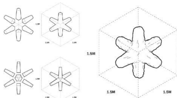
Figure 06. base Module “Tetrapod” Aggregate geometry breakdown.
