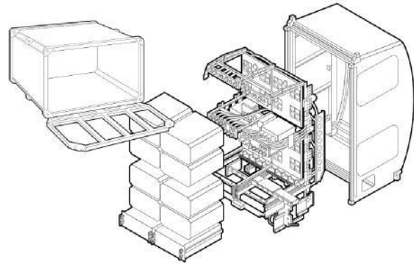
Figure 15. Technical diagram of ISPR. Standard Payload Racks Research payload within the U.S., European, and Japanese laboratories typically are housed in a standard rack, such as the International Standard Payload Rack (ISPR). Image: NASA
