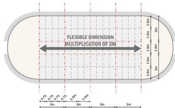
Figure 16. Floorplan, Organising Grid of 4-bay Habitable Module
