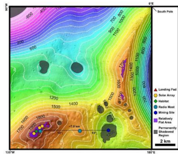
Figure 2. Topographic Contour Map of the Lunar South Polar Ridge (McCanaan, et al, 2019)
