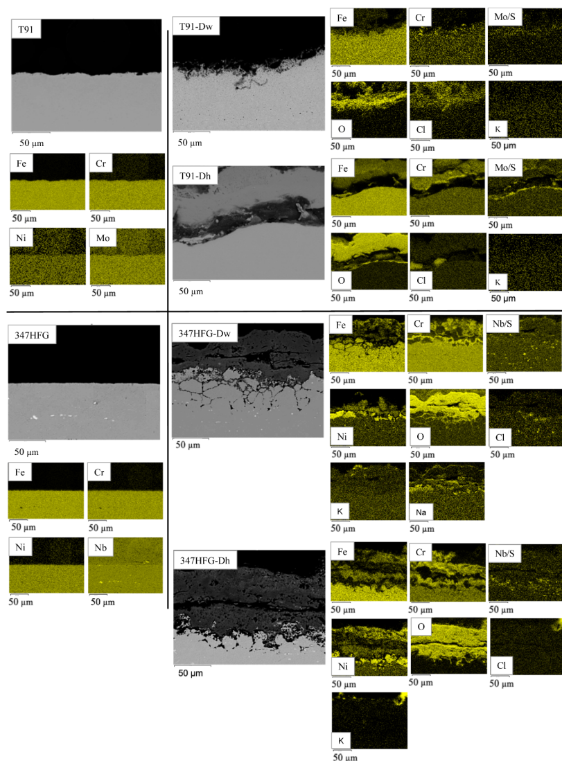
Fig. 7. BSE images (grey-scale) and EDX mappings (yellow-scale) of T91 (top) and 347HFG (bottom). Unexposed reference images of both alloys are on the left. EDX peak overlaps on 347HFG and T91 have been identified for Nb/S and Mo/S respectively. Samples with deposit following 1000 h exposure in WWF test gas conditions at 600 °C and a deposition flux of 100 \mu\text{g}/\text{cm}^2\text{h} are shown on the right. (For interpretation of the references to colour in this figure legend, the reader is referred to the web version of this article.)
