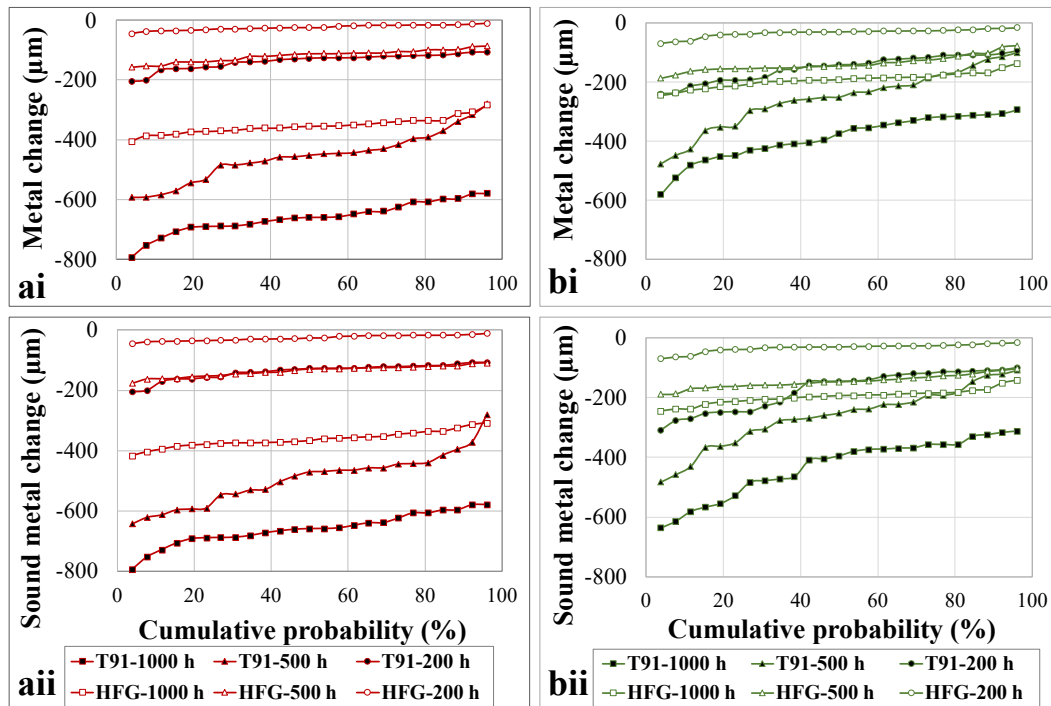
Fig. 5. Cumulative probability plots showing distributions of metal and sound metal changes (i & ii respectively) measured along the cross-sectioned T91 and 347 HFG sample planes. The further away the plot is from the x-axis, the greater the metal loss is. Samples have been exposed to deposits (a) Dw and (b) Dh in WWF test gas conditions at a deposit flux of 100 \mu\text{g}/\text{cm}^2\text{h} .
