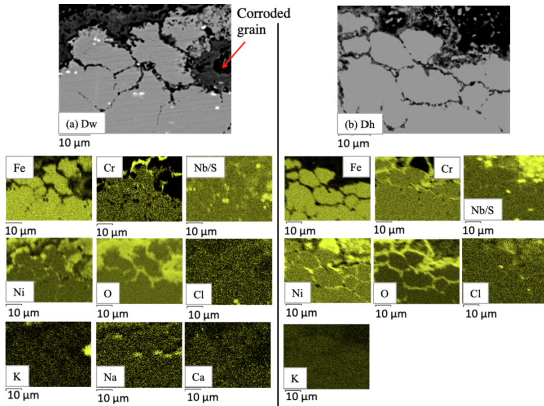
Fig. 8. Grain boundary damages on 347HFG samples exposed to (a) Dw and (b) Dh at flux 50 µg/cm 2 h for 500 h in WWF test gas conditions at 600 °C.
