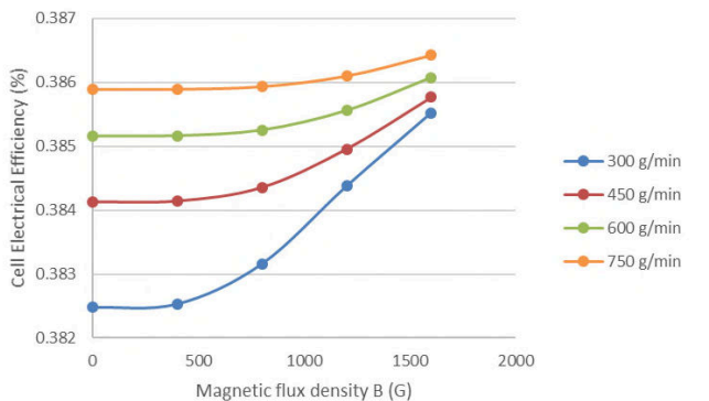
Fig. 6: Cell electrical efficiency vs. Magnetic flux density curves
