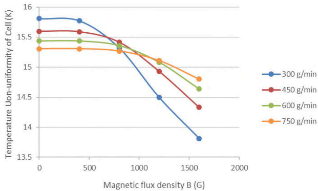
Fig. 5: Cell temperature non-uniformity vs, Magnetic flux density curves
