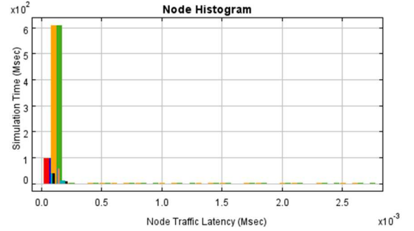
Figure 13: Decreased Latency in Network A and B.
