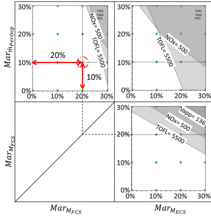
Fig. 15 Feasible margin space for point B when Mar_{M_{FCS}} = 20\% and Mar_{\dot{m}_{perOcp}} = 10\% .
