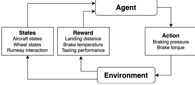
Figure 3. AI-based braking states, actions and rewards
