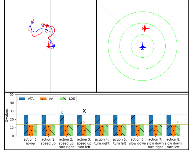
Fig. 3. Trained RL agent tracking performance. The upper left plot is a bird's eye view. The upper right figure is perspective from the blue agent body frame and each green circle has a 1,000 m radius. The lower figure is decomposed reward bar chart, the black x sign represents the chosen action while the other x signs represent the action associated with the maximum expected reward of each DQN for their respective reward type.
