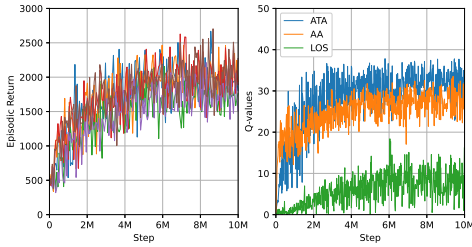
Fig. 2. Left: Episodic return of multiple training. Right: Comparison of component Q-values of multiple training.
