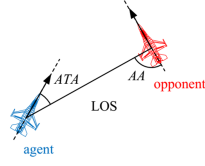
Fig. 1. ATA, AA, and LOS geometric representation.
