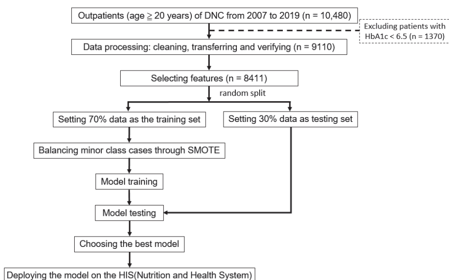
Figure 1. Research flowchart.
