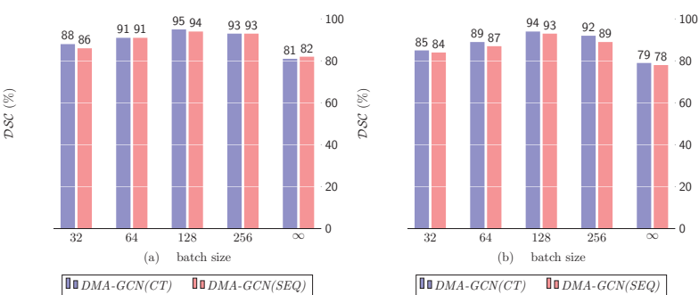
Figure 16. Cartilage DSC(\%) score vs. batch size. (a) Femoral cart, (b) tibial cart.
