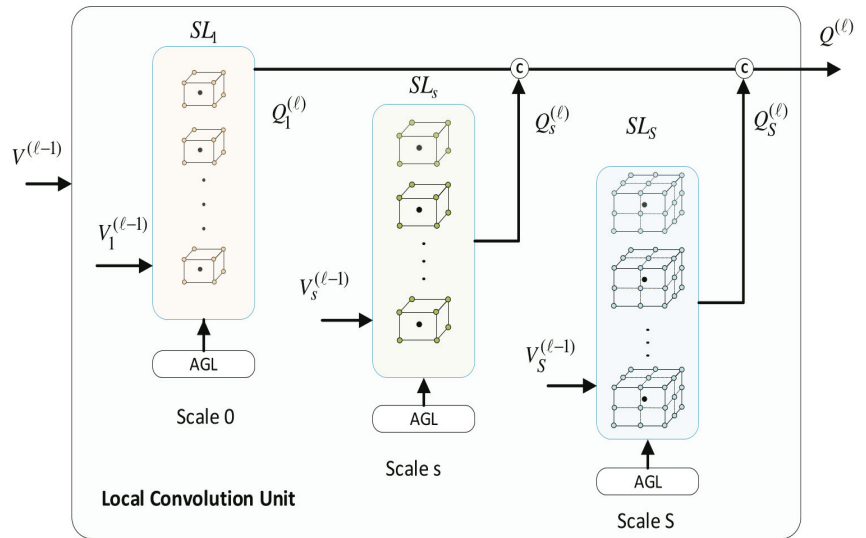
Figure 7. Detailed description of the local convolutional unit, which aggregates local contextual information from node neighborhoods at different spatial scales.
