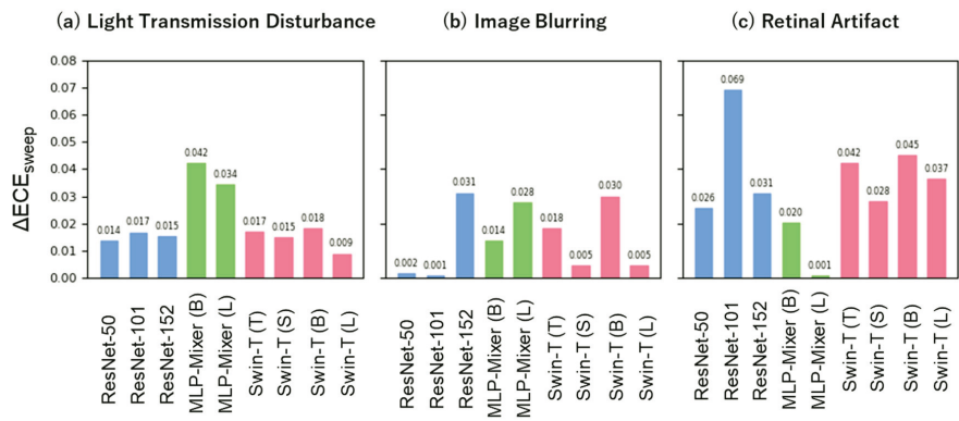
Figure 6. Robustness for calibration ability under three unique distribution shifts. The x-axis depicts each model architecture with different model size. The blue, green, and red bars represent the ResNet, MLP-Mixer, and Swin-Transformer architectures, respectively. The y-axis represents the difference in ECE sweep between distribution shift and in-distribution.
