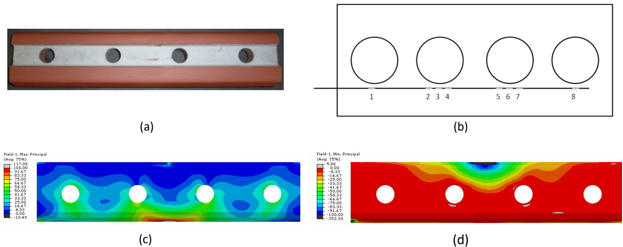
Figure 4. (a) The fishplate (b) the location of the FBG sensors, where the numbers are used to identify the individual sensors. (c) Maximum principal strain and (d) minimum principal strain distributions predicted by finite element modelling.
