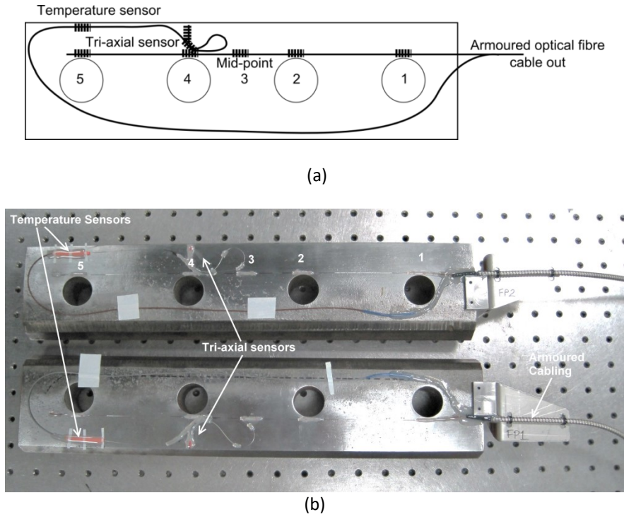
Figure 3. (a) Schematic illustrating the location of the optical fibre Bragg grating strain and temperature sensors [14]. (b) Photograph of the instrumented fishplates [14]. The dimensions of the fishplates are 40mm x 90mm x 400 mm.
