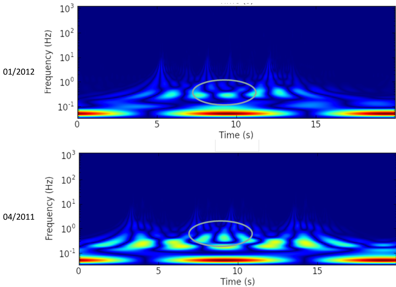
Figure 18. CWT of the strain measured by the sensor, highlighted in the “nose array” in figure 15, on PS1 Left in April 2011 and January 2012.
