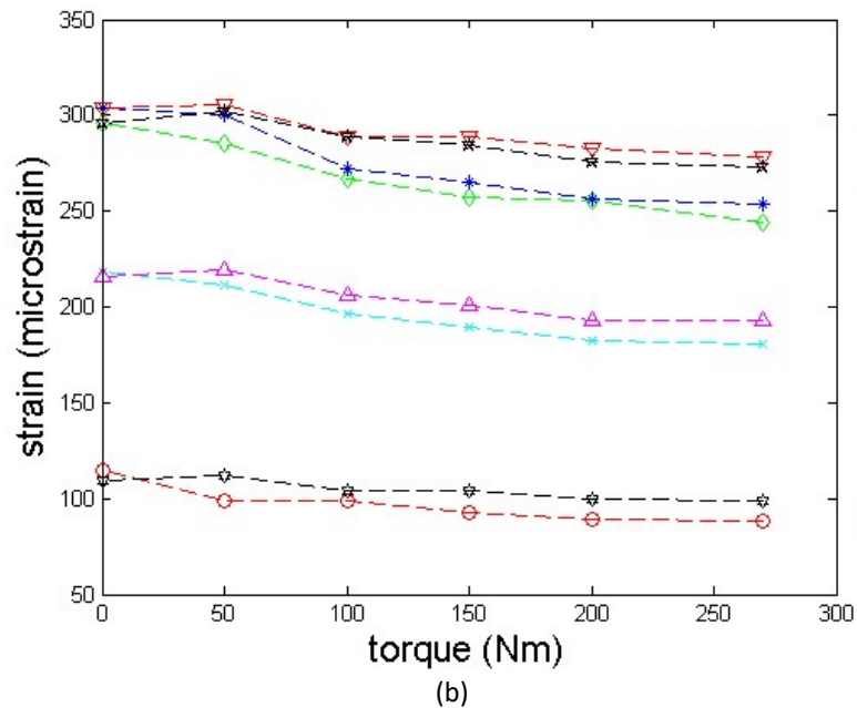
Figure 6. Results from the 4-point bending of a fishplate joint. (a) The strain profile measured using a fibre optic sensor array (the dashed line is a guide to the eye, and the numbers indicate the sensors) when all bolts were at the same torque, 270 Nm. The locations of the sensors are measured relative to the left hand edge of the fishplate. (b) The strains measured for a 40 kN applied load when the torque of the left-hand inner bolt (adjacent to sensors 2, 3 and 4) was varied. The numbers refer to the sensor locations, identified in figure 6 (b).
