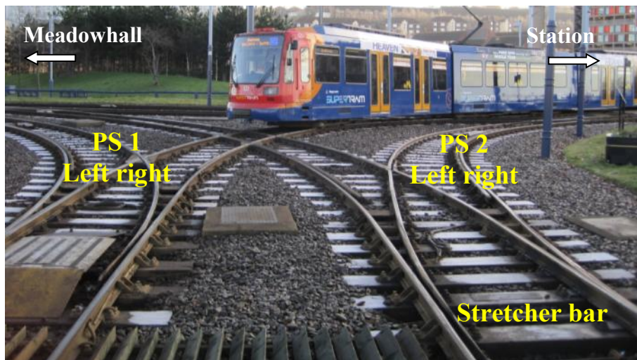
Figure 13. Configuration of the instrumented switchblades and stretcher bar on the Delta. The photograph was taken looking from the city bridge. “Meadowhall” and “Station” are significant stations on the network, and are included to allow the direction of travel of the crossing tram to be distinguished. “PS1 Left”, “PS1 Right”, “PS2 Left” and “PS2 Right” are used to identify the switch blades in the text. .
