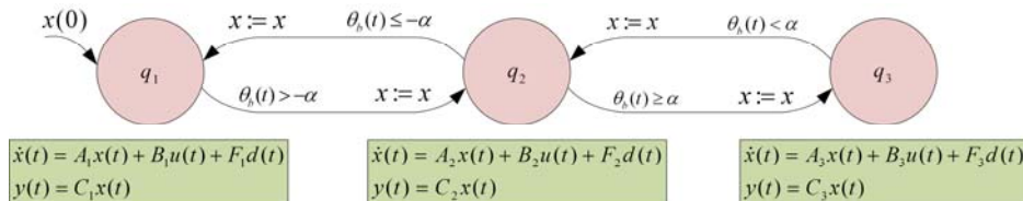
Fig. 5. Hybrid automata of the electric powertrain dynamics.
