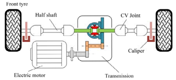
Fig. 1. Overall structure of the electric powertrain system.
