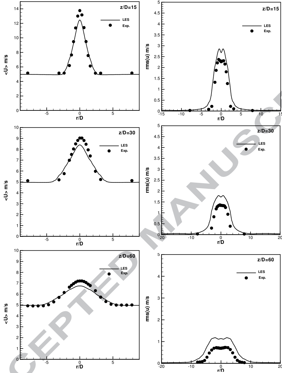
Fig.2. Comparison of the mean (left-hand side) and rms (right-hand side) axial velocity . Lines represent LES results, and symbols represent experimental measurements
