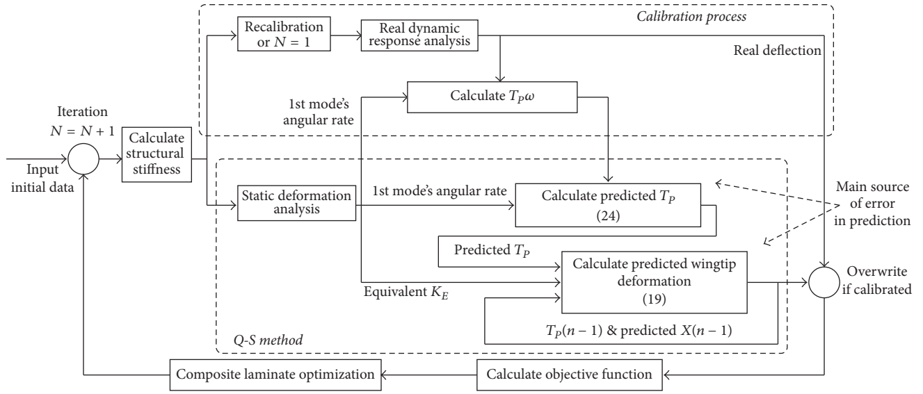
FIGURE 2: The flowchart of the Q-S method in structure optimization procedure.
