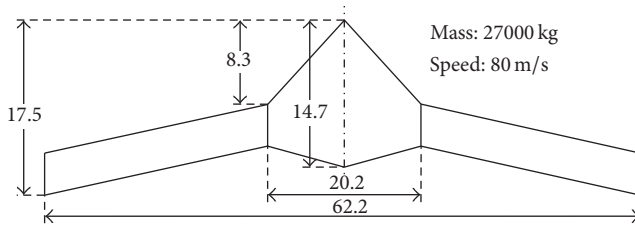
FIGURE 3: Planform of a flying wing aircraft model (unit: m).
