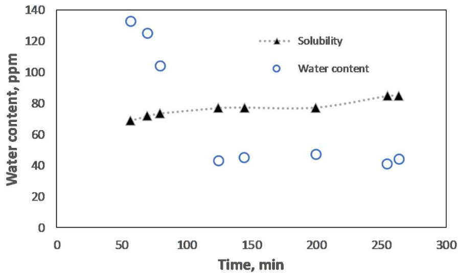
Fig. 10 Measured water content in fuel by KF coulometer and its solubility at different temperatures
