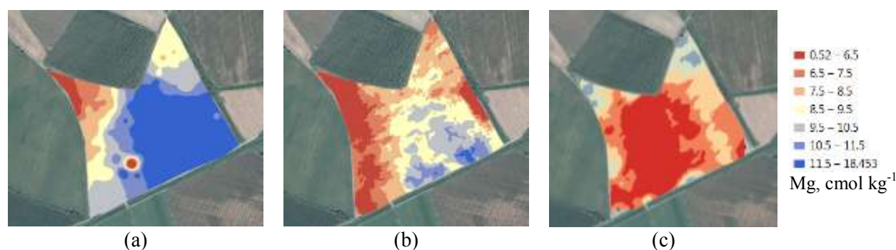
Figure 8. Mg Comparison maps: (a) laboratory-measured based on 92 samples, (b) on-line Vis-Nir predicted (6486 points) measured in 2013, and (c) on-line Vis-Nir predicted (2496 points) measured in 2015.
