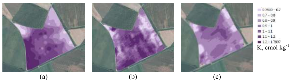
Figure 7. K Comparison maps: (a) laboratory-measured based on 92 samples, (b) on-line Vis-Nir predicted (6486 points) measured in 2013, and (c) on-line Vis-Nir predicted (2496 points) measured in 2015.
