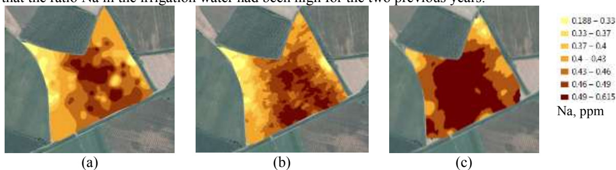
Figure 6. Na Comparison maps: (a) laboratory-measured, based on 92 samples, (b) on-line Vis-Nir predicted (6486 points) measured in 2013, and (c) on-line Vis-Nir predicted (2496 points) measured in 2015.
