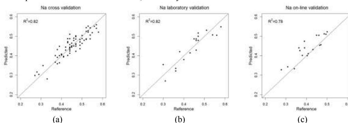
Figure 3. The scatter plots of measured versus predicted Na for laboratory and on-line predictions.
