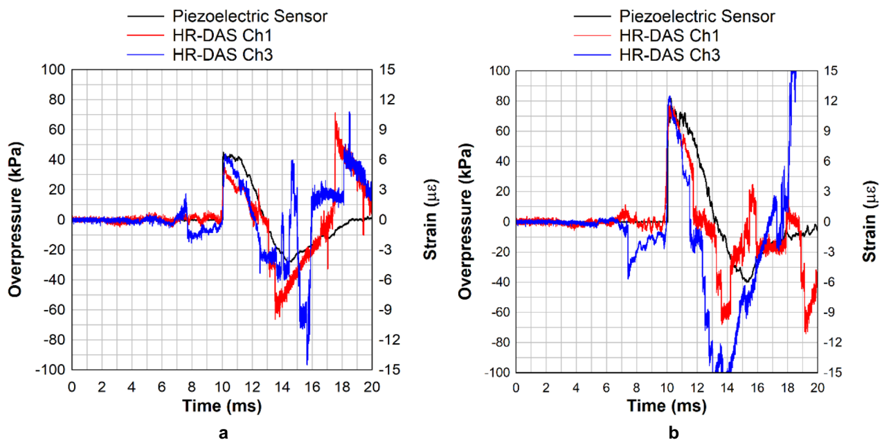
Fig. 10 Overlaid overpressure and strain histories measured by the piezoelectric transducer and HR-DAS sensors. a Test no. 25: 125- \mu\text{m} Mylar, i.e., p_{\text{so}} = 45 \text{ kPa} . b Test no. 28: 250- \mu\text{m} Mylar, i.e., p_{\text{so}} = 72 \text{ kPa}
