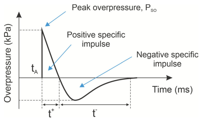
Fig. 1 Incident/side-on overpressure–time history of an idealised blast wave
