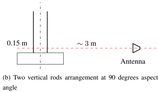
Fig. 5: Experimental setup
