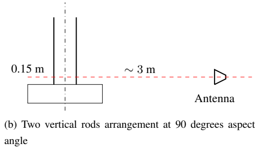
Fig. 5: Experimental setup
