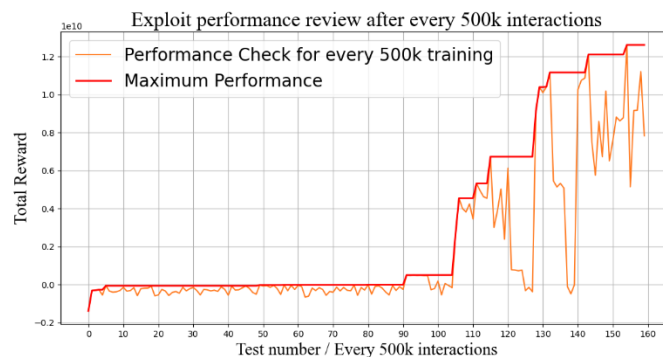
Fig. 4. Reward trend
