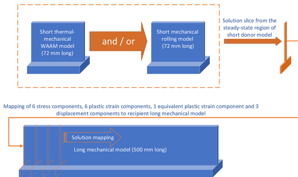
Figure 1. Schematic diagram of the proposed efficient modelling approach for determining steady-state thermal–mechanical variables using short models of WAAM and rolling, followed by mapping solution to long model for further analysis.
