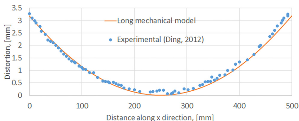
Figure 12. Validation of out-of-plane distortion prediction by the mapped long mechanical model after clamps removal. Note that the experimental measurement by Ding [23] was based on a four-layer deposited wall, and the WAAM model was adapted accordingly. The distortion measurement was conducted on the substrate bottom using a Romer omega arm with R-scan 3D laser scanning system [23].
