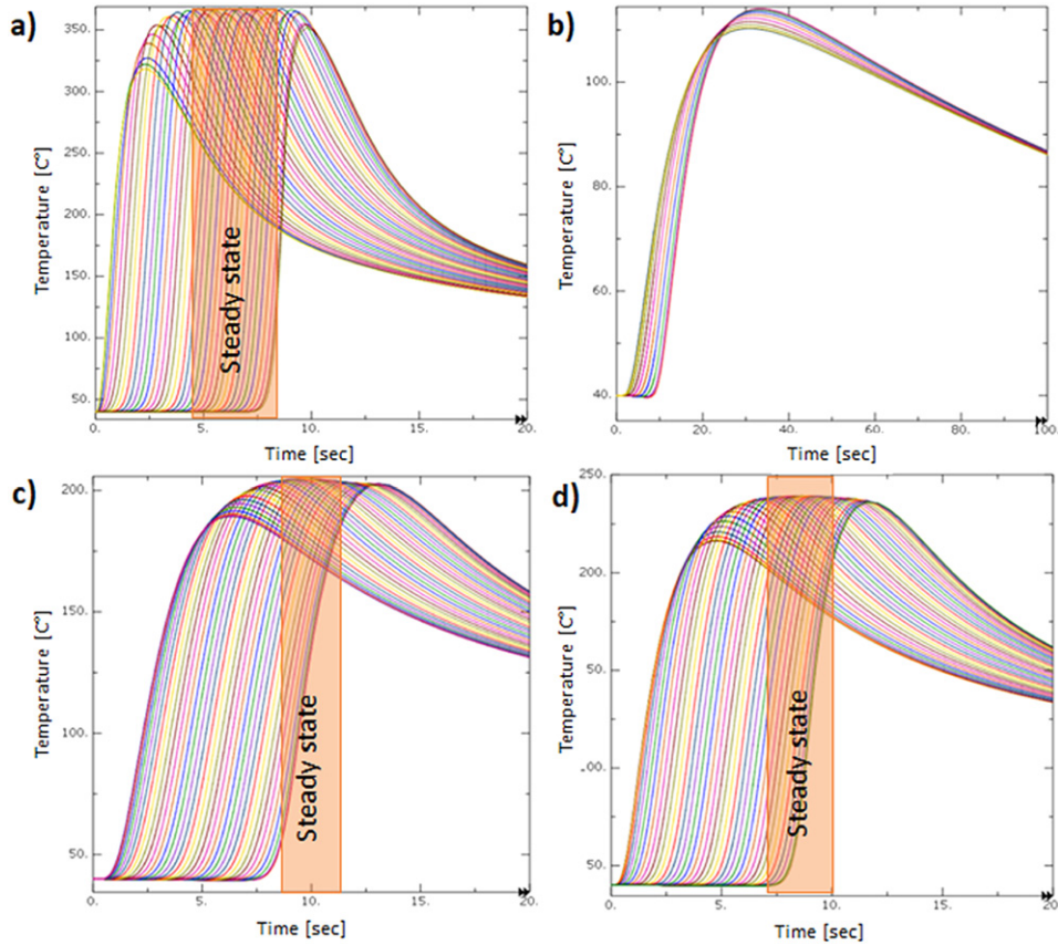
Figure 6. Predicted temperature histories at different longitudinal locations (i.e. different X coordinates) which are coincident with (a) TP1, (b) TP2, (c) TP3 and (d) TP4 in the YZ plane (see figure 2 for locations of TP1–TP4). Note that the peak temperatures corresponding to steady state of the WAAM deposition are highlighted.
