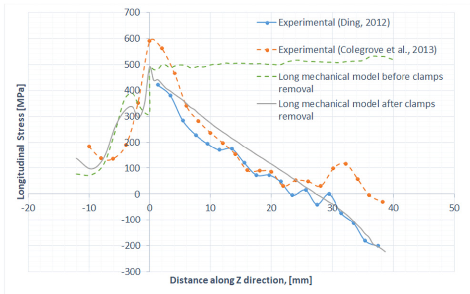
Figure 11. Longitudinal RS distributions along the Z-direction (with distance from the upper surface of the substrate, see figure 10(c) for the path of the line plots) in the mapped long mechanical model before and after clamps removal for the WAAM component. The experimental measurements by Ding [23] and Colegrove et al [5] are also included, which were conducted using neutron diffraction method after clamps removal.
