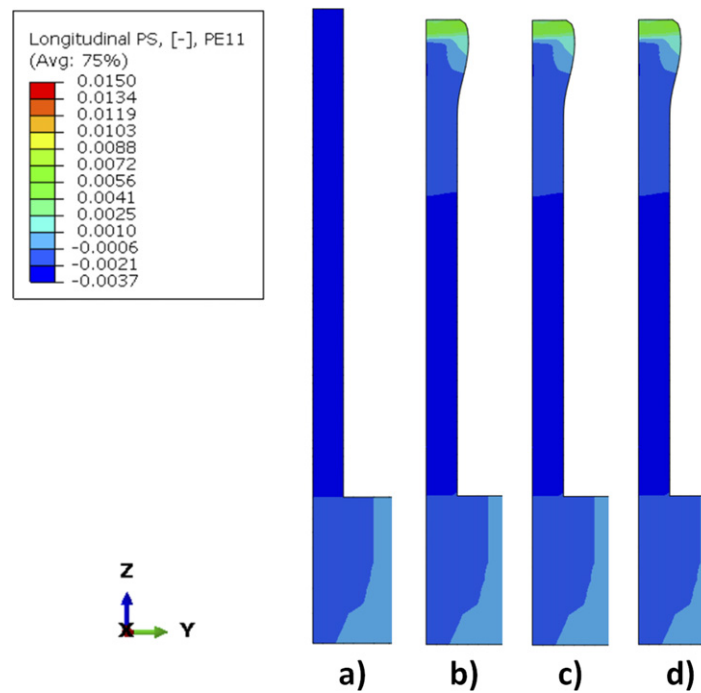
Figure 16. Predictions of longitudinal PS distributions in the steady-state region for the combined WAAM and rolling process: (a) short model with clamps before rolling; (b) short model with clamps after rolling; (c) mapped long model with clamps; (d) mapped long model after clamps removal.
