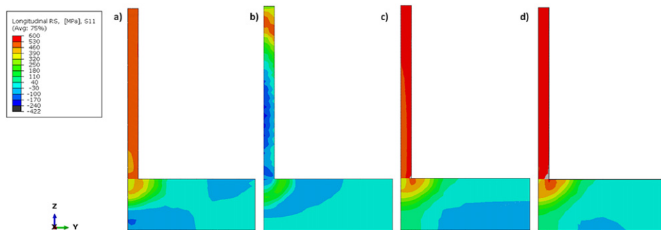
Figure 9. Cross-sectional distributions of longitudinal RS in the steady-state region for the WAAM: (a) full-size mechanical model [23]; (b) short mechanical model with free ends; (c) short mechanical model with constrained ends; (d) short mechanical model with full longitudinal constraint.
