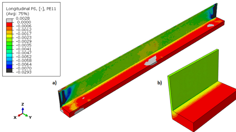
Figure 8. 3D distributions of the longitudinal PS for the WAAM: (a) full-size mechanical model [23]; (b) short mechanical model with full longitudinal constraint.
