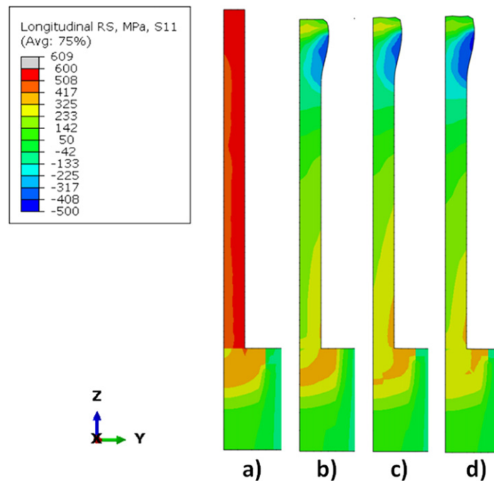
Figure 17. Predictions of longitudinal RS distributions in the steady-state region for the combined WAAM and rolling process: (a) short model with clamps before rolling; (b) short model with clamps after rolling; (c) mapped long model with clamps; (d) mapped long model after clamps removal.
