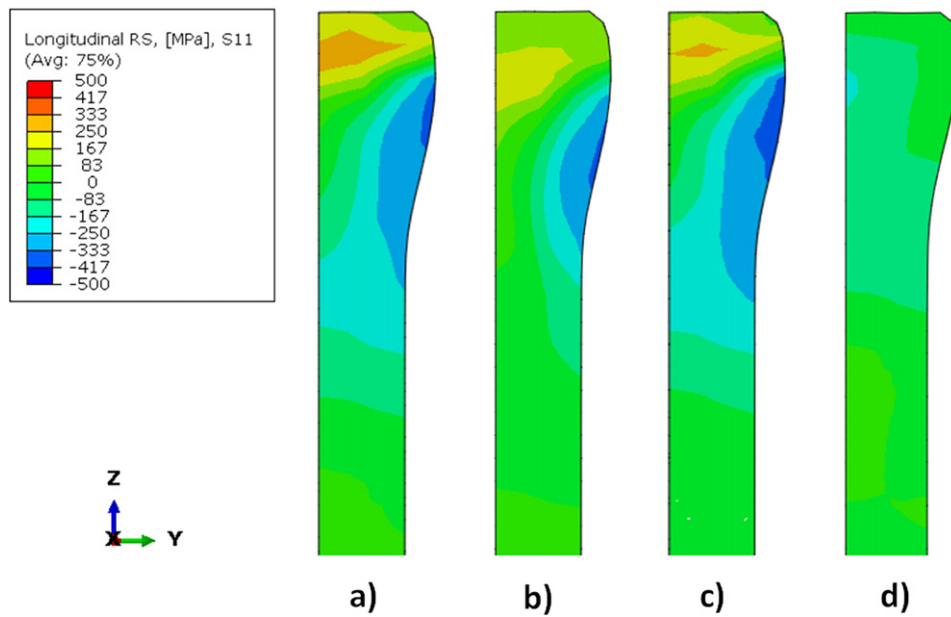
Figure 14. Comparison of predicted longitudinal RS distributions in the steady-state region of high pressure rolling: (a) conventional full-size model; (b) short model with free ends; (c) short model with constrained ends; (d) short model with full longitudinal constraint. Adapted from [39]. CC BY 4.0.
