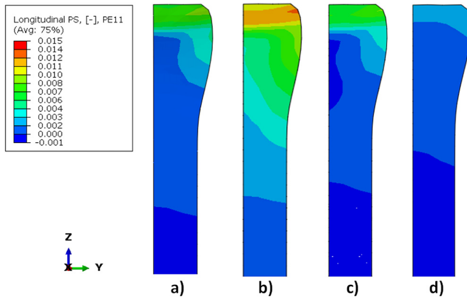
Figure 13. Comparison of predicted longitudinal PS distributions in the steady-state region of high pressure rolling: (a) conventional full-size model [39]; (b) short model with free ends; (c) short model with constrained ends [39]; (d) short model with full longitudinal constraint.
