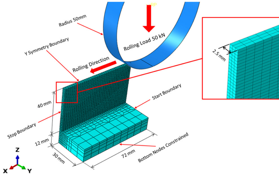
Figure 4. Short rolling model for a wall component with identical geometry to the WAAM component (figure 2). Adapted from [39]. CC BY 4.0.
