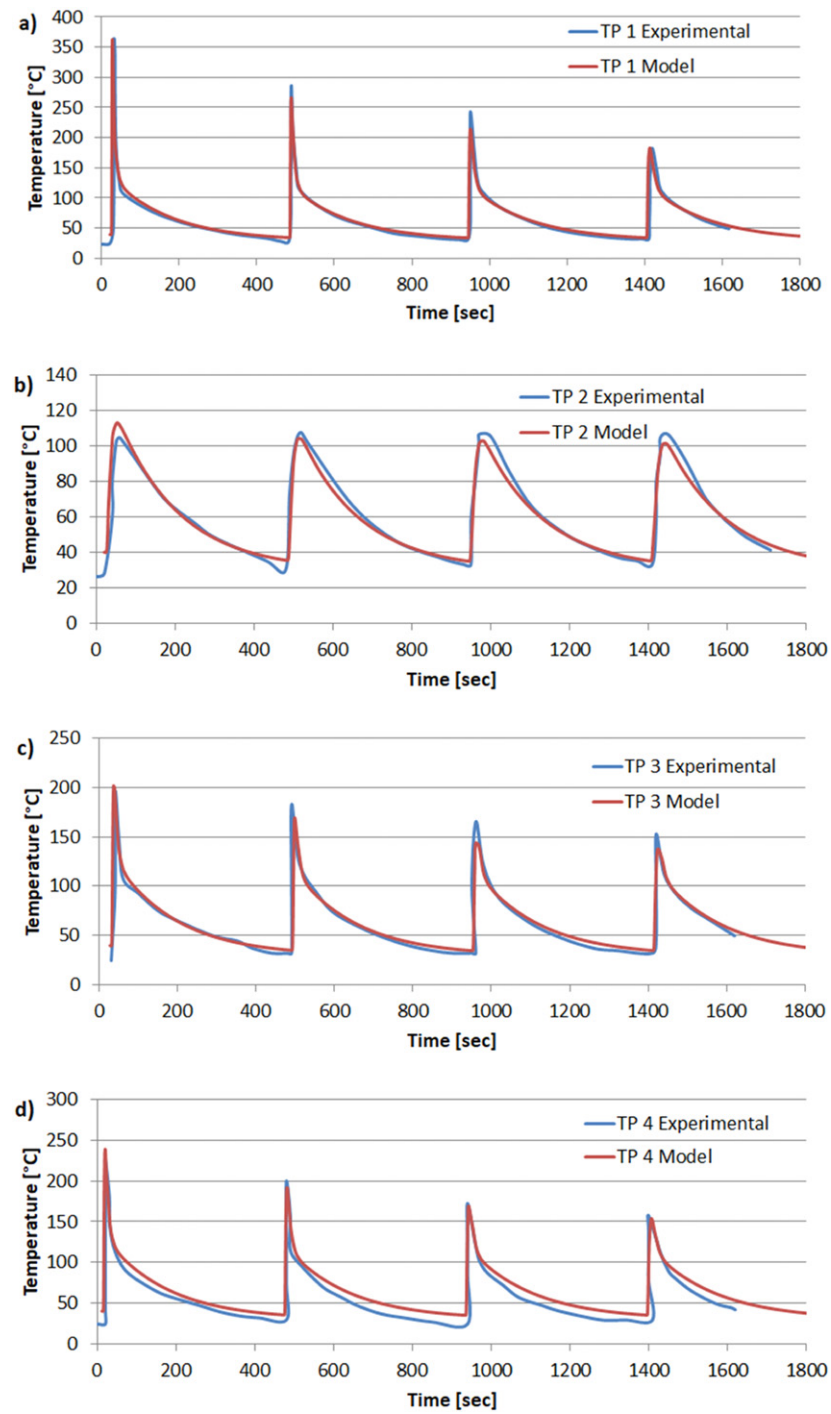
Figure 5. Temperature histories predicted by the short WAAM thermal model at the thermocouple locations: (a) TP1, (b) TP2, (c) TP3 and (d) TP4. The experimental measurements by Ding [23] are also included for comparison.
