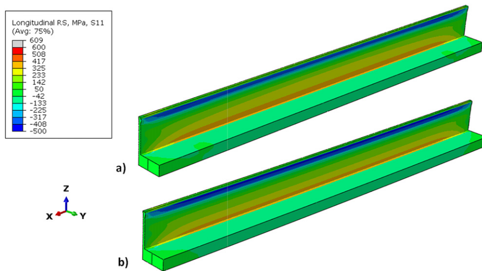
Figure 18. 3D distributions of longitudinal RS predicted by the mapped long mechanical model for the combined process of WAAM and rolling: (a) before clamps removal; (b) after clamps removal (a deformation scale factor of 5 is used to improve visibility of distortion).
