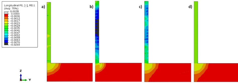
Figure 7. Cross-sectional distributions of longitudinal PS in the steady-state region for the WAAM: (a) full-size mechanical model [23]; (b) short mechanical model with free ends; (c) short mechanical model with constrained ends; (d) short mechanical model with full longitudinal constraint.
