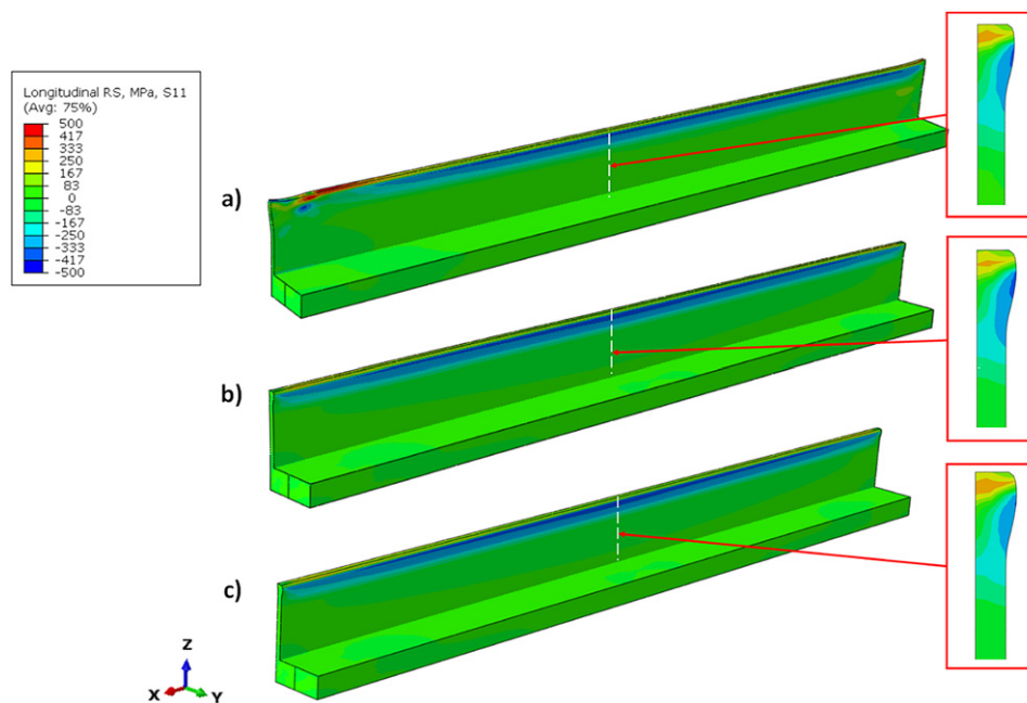
Figure 15. Longitudinal RS distributions predicted by the long mechanical model for the high pressure rolling: (a) conventional full-size model under clamped condition [39]; (b) mapped model under clamped condition; (c) mapped model after clamps removal (a deformation scale factor of 5 is used to improve visibility of distortion). The RS distributions in the middle-length section are also shown.
