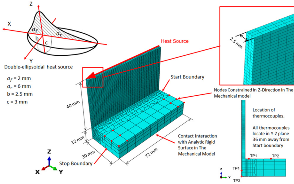
Figure 2. Short transient thermal–mechanical model of 20-layer WAAM-deposited wall with reduced length compared to the samples in previous experiments [20, 23]. The schematic of double-ellipsoidal heat source is also shown. The coordinates (in mm) of the thermocouples are TP1 (36, 5, 12), TP2 (36, 20, 12), TP3 (36, 0, 0) and TP4 (36, 0, 4). The Y coordinate of the symmetry plane and the Z coordinate of the substrate bottom are both zero.
