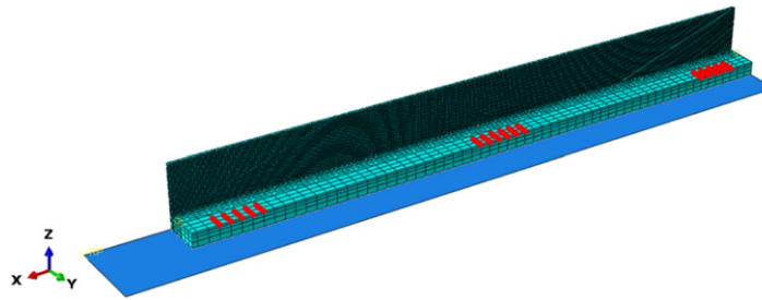
Figure 3. Mapped long mechanical model to simulate the removal of clamps (the constrained nodes representing the clamps are indicated in red).
