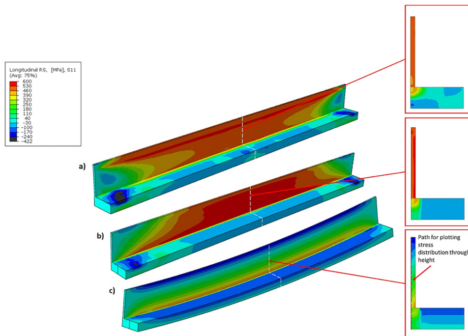
Figure 10. Longitudinal RS distributions predicted by the long mechanical models for the WAAM: (a) conventional full-size model under clamped condition [23]; (b) mapped model under clamped condition; (c) mapped model after clamps removal (a deformation scale factor of 5 is used to improve visibility of distortion). The RS distributions in the middle-length section are also shown.
