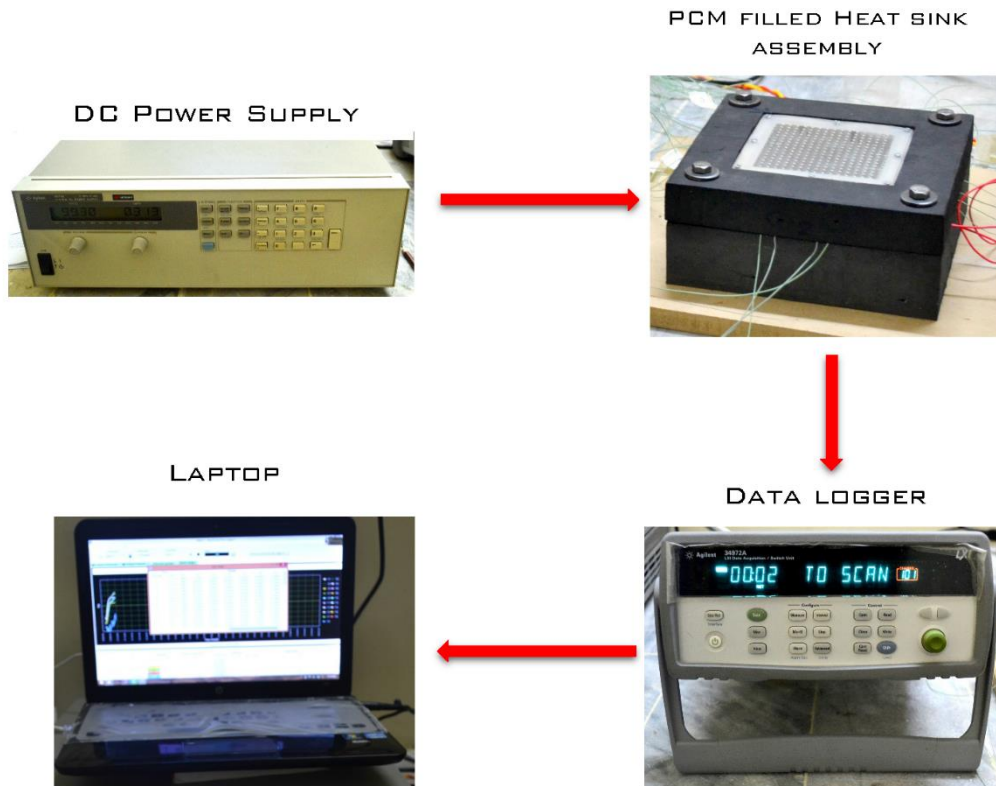
Figure 1b-Line flow of experimental facility.
