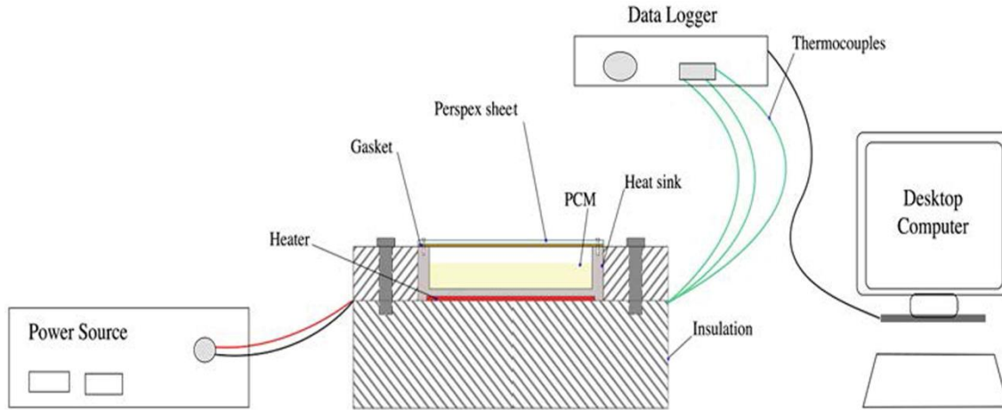
Figure 1a-Schematic diagram of experimental setup.
