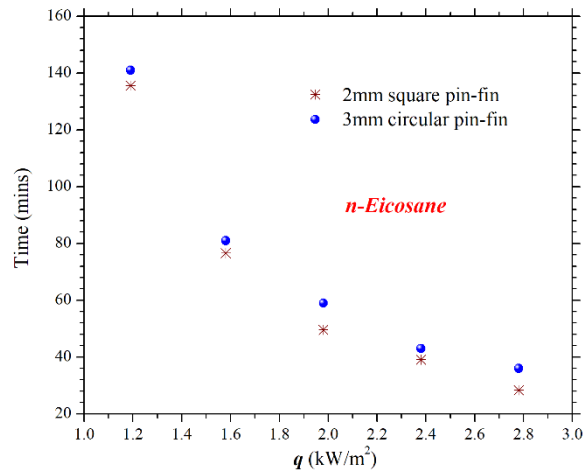
Figure 3-comparison of latent heating phase completion time.
