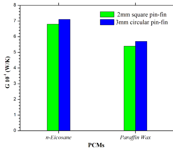
Figure 6-Comparison of thermal conductance of heat sinks for paraffin wax and n-eicosane .
