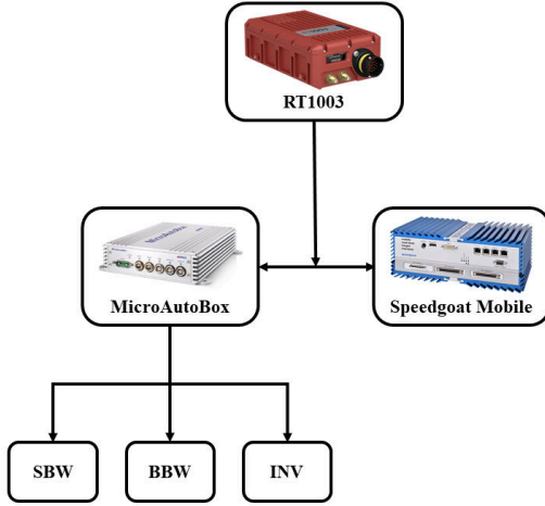
Fig. 4. Hardware topology of the testing vehicle for data processing.
