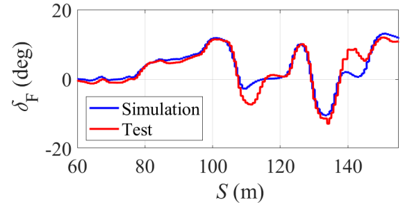
Fig. 12. Front steering commands
