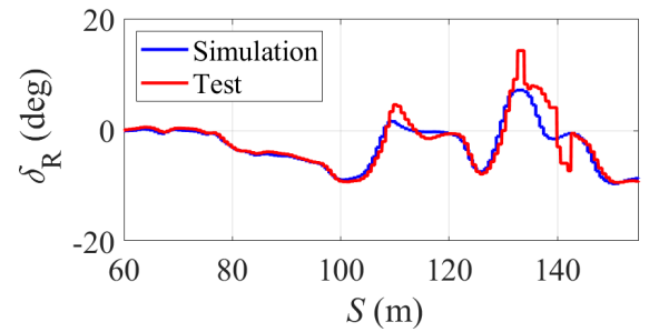
Fig. 13. Rear steering commands
