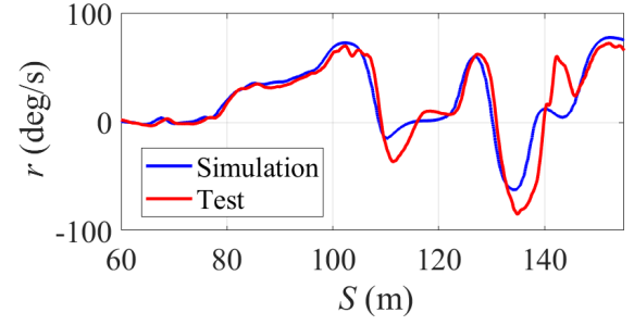
Fig. 11. Yaw rate
