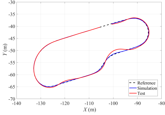
Fig. 6. Vehicle trajectory
