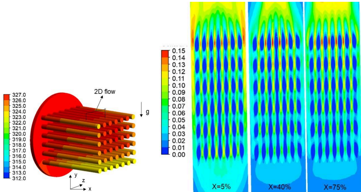
Figure 5 a) Temperature (K) distribution and (b) velocity (m/s) field at different axial locations on a passively cooled pin fin heat sink
