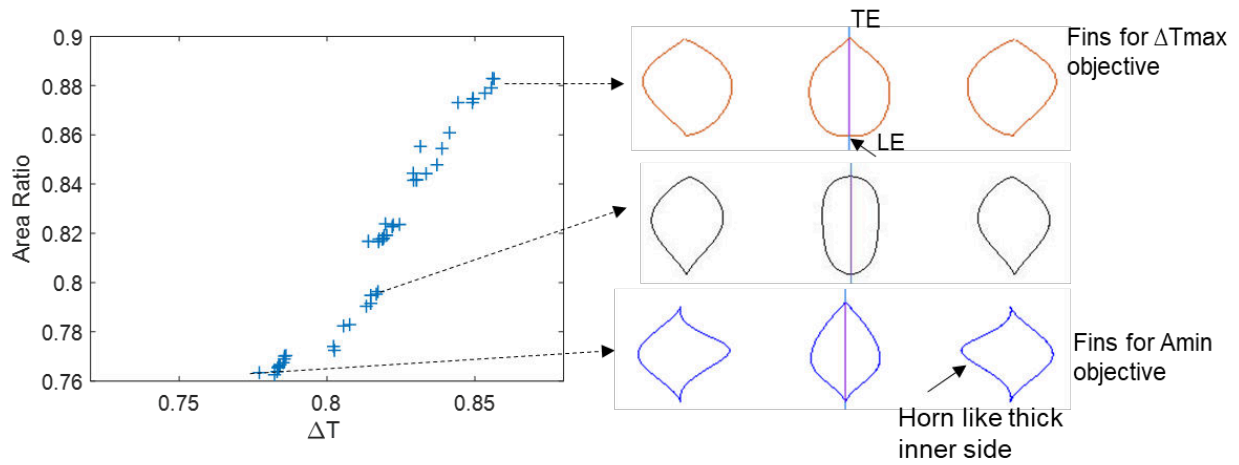
Figure 10 Pareto optimal front obtained for bottom row fin shape optimisation ( H/D=0.83 )
