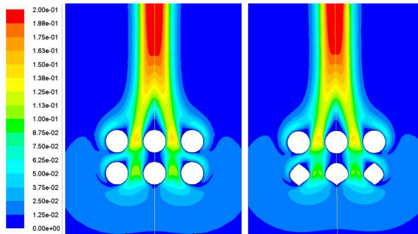
Figure 17 velocity (m/s) field comparison between circular fins and optimised ( \Delta T_{\max} objective) bottom row fins
