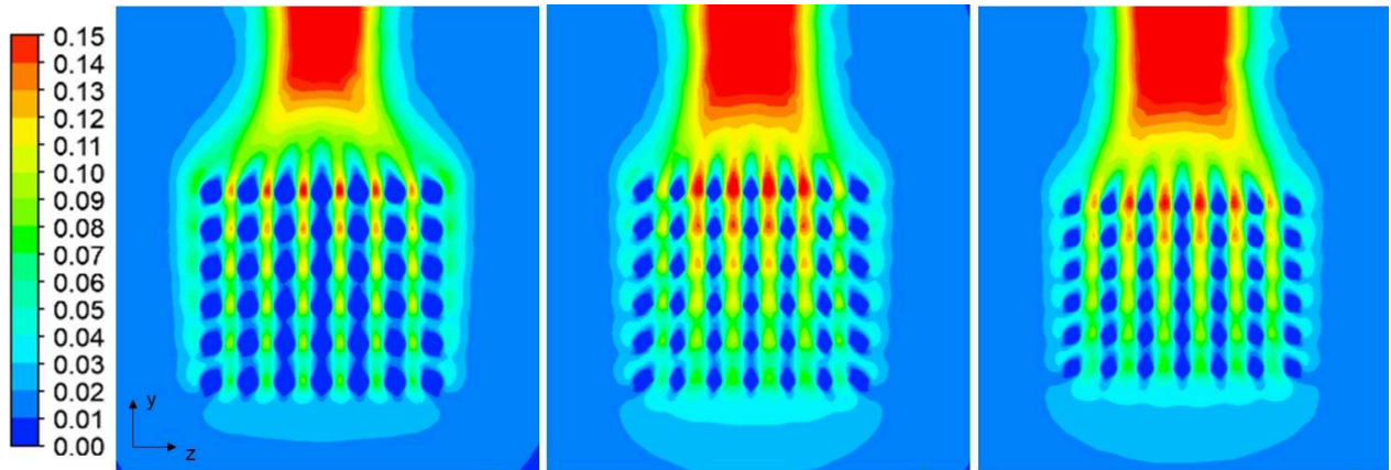
Figure 21 Velocity (m/s) field at mid-length of heat sink A, optimised heat sink, and heat sink B.
