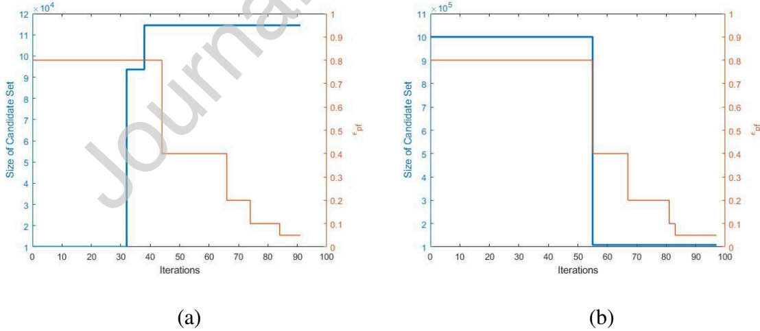
Figure 3 Update history of candidate size: (a) n_{initial} = 10^4 , (b) n_{initial} = 10^6
