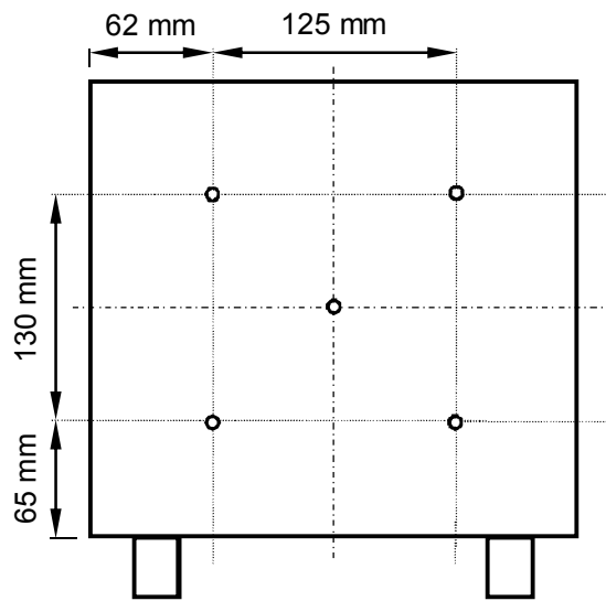
Figure 9. Schematic location of the surface static pressure tappings used to evaluate base pressure on the vehicle. Adapted from Velikov (2009)
