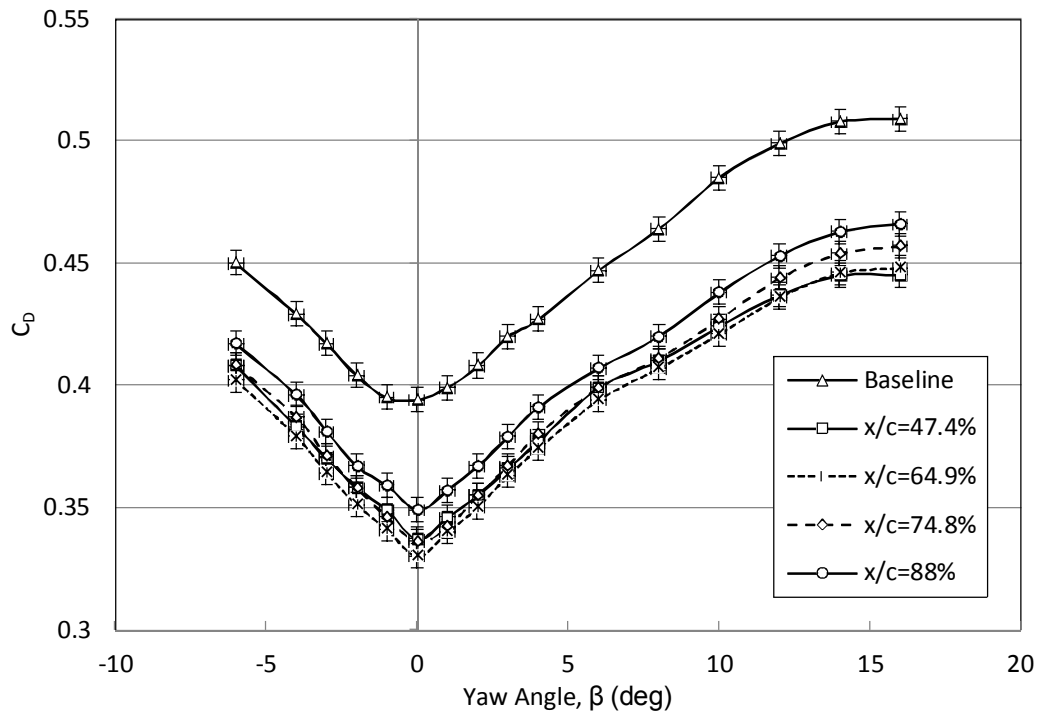
Figure 4. The effect of introducing roof curvature (magnitude of maximum roof curvature profile depth fixed) on the variation of drag coefficient with yaw angle.
