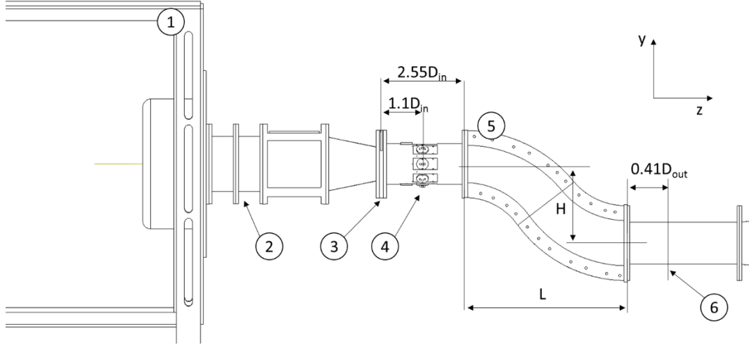
Fig. 1: Cranfield test facility schematic: 1- seeding chamber, 2- flow conditioning section, 3- honeycomb screen section, 4- pressure measurements ports, 5- S-duct, 6- measurement plane (AIP).
