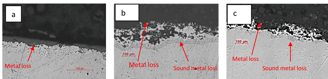
Figure 4. Optical images of cross-sections through alloy CMSX-4 (a) and IN713LC (b) covered with sodium chloride deposits exposed to air + 300 vppm \text{SO}_x gaseous atmosphere gas for 240 h and C1023 (c) covered with sodium chloride deposits exposed to air + 300 vppm \text{SO}_x gaseous atmosphere gas for 160 h at 900°C.
