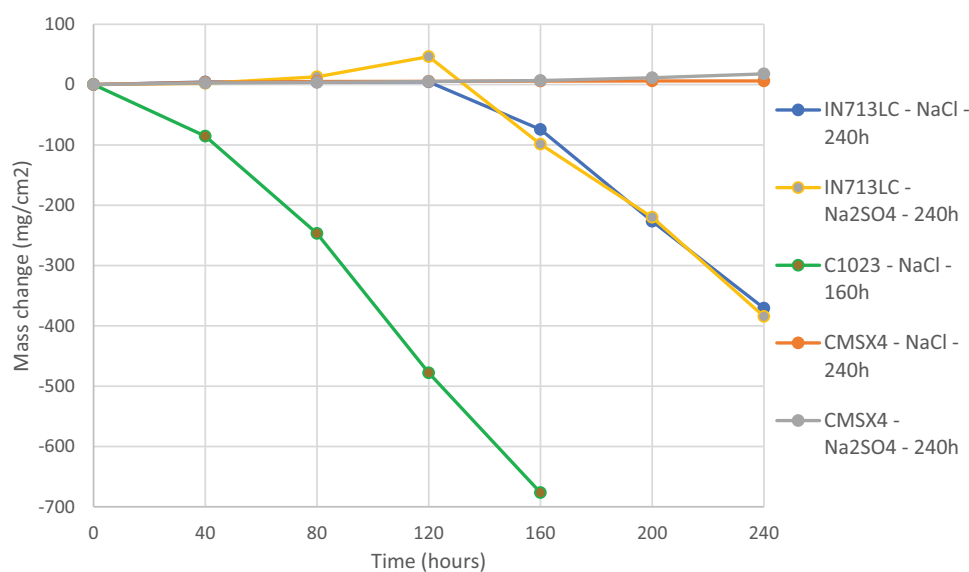
Figure 2. Mass change data of alloys IN713LC, C1023, and CMSX-4 covered with salts deposits exposed to air + 300 vppm \text{SO}_x gaseous atmosphere gas for 160 and 240 h at 900°C.
