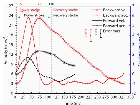
Fig. 3. The speed and acceleration of the diving beetle during straight forward swimming and straight backward swimming. Where “vel.” and “acc.” are the abbreviations of velocity and acceleration, respectively.
