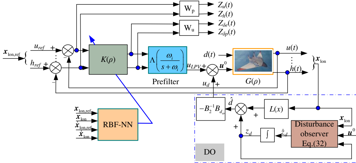
Fig. 3. Block diagram of the DO-NNLPV controller for the BWB aircraft
