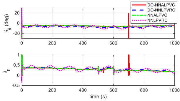
Fig.15 Control inputs of the elevator and thrust
